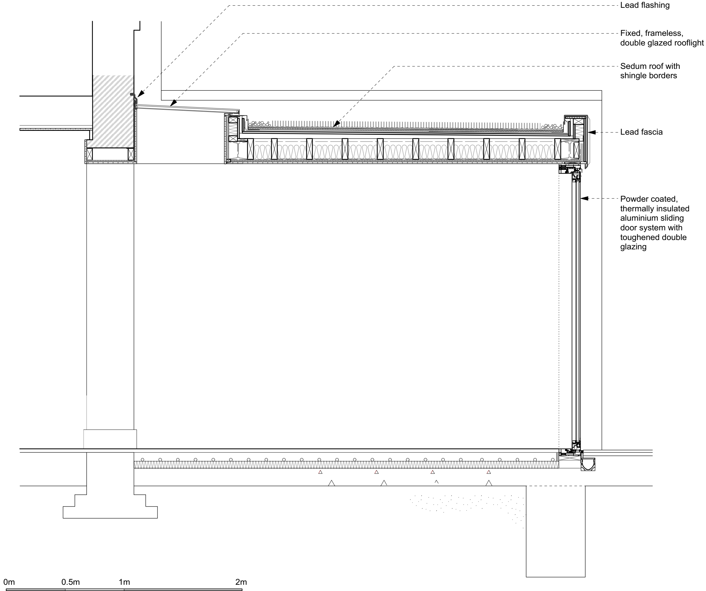
Proposed DETAILS _ Conservatory Extension_ Section I
