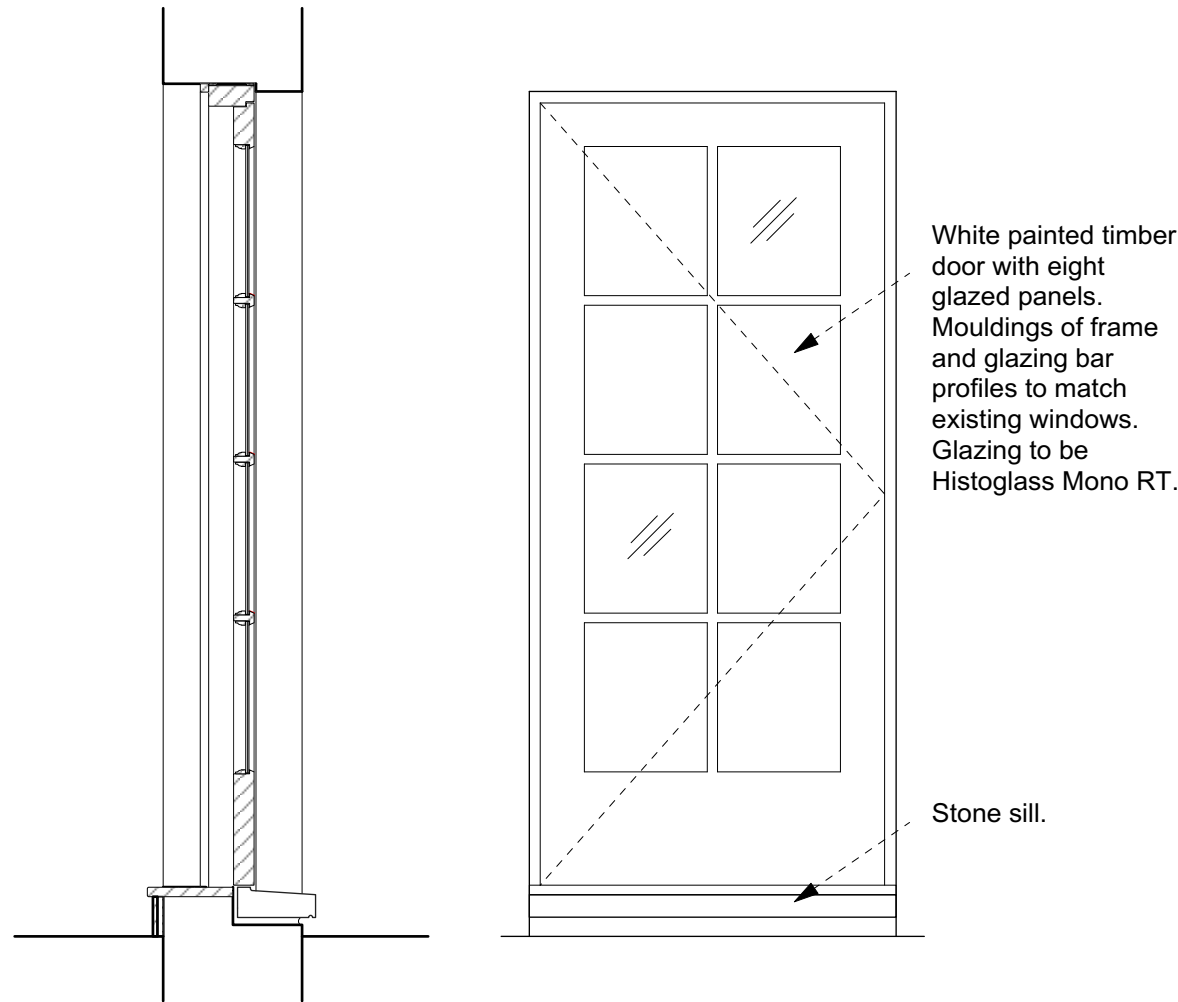
Section 1:20
