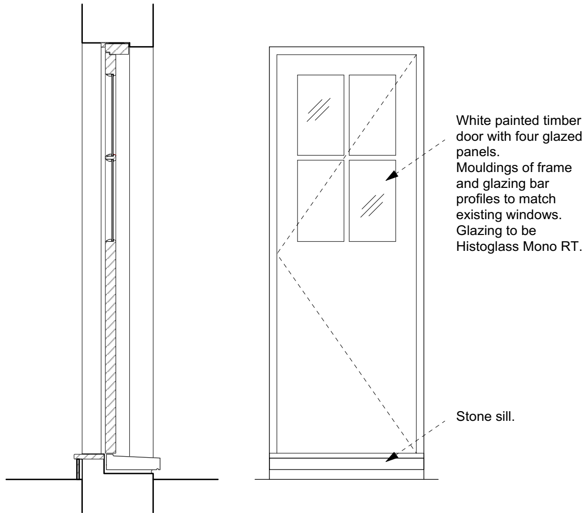
Section 1:20
