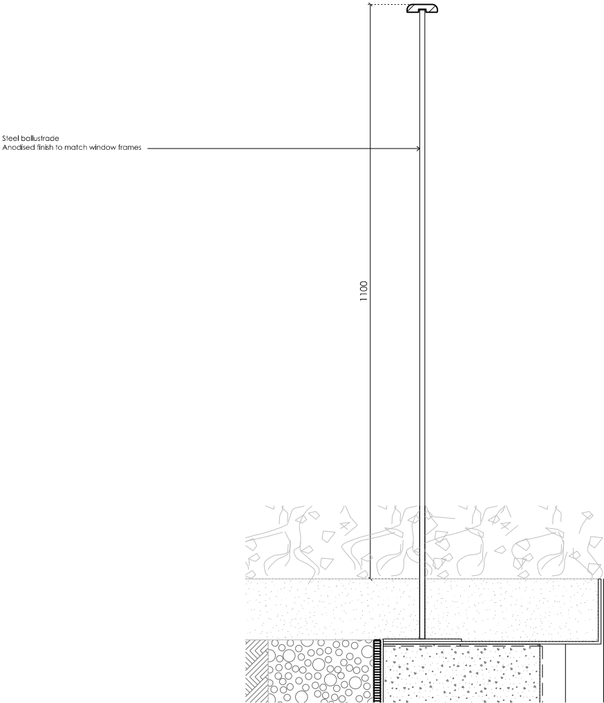
Ballustrade Connection Detail 1:10
