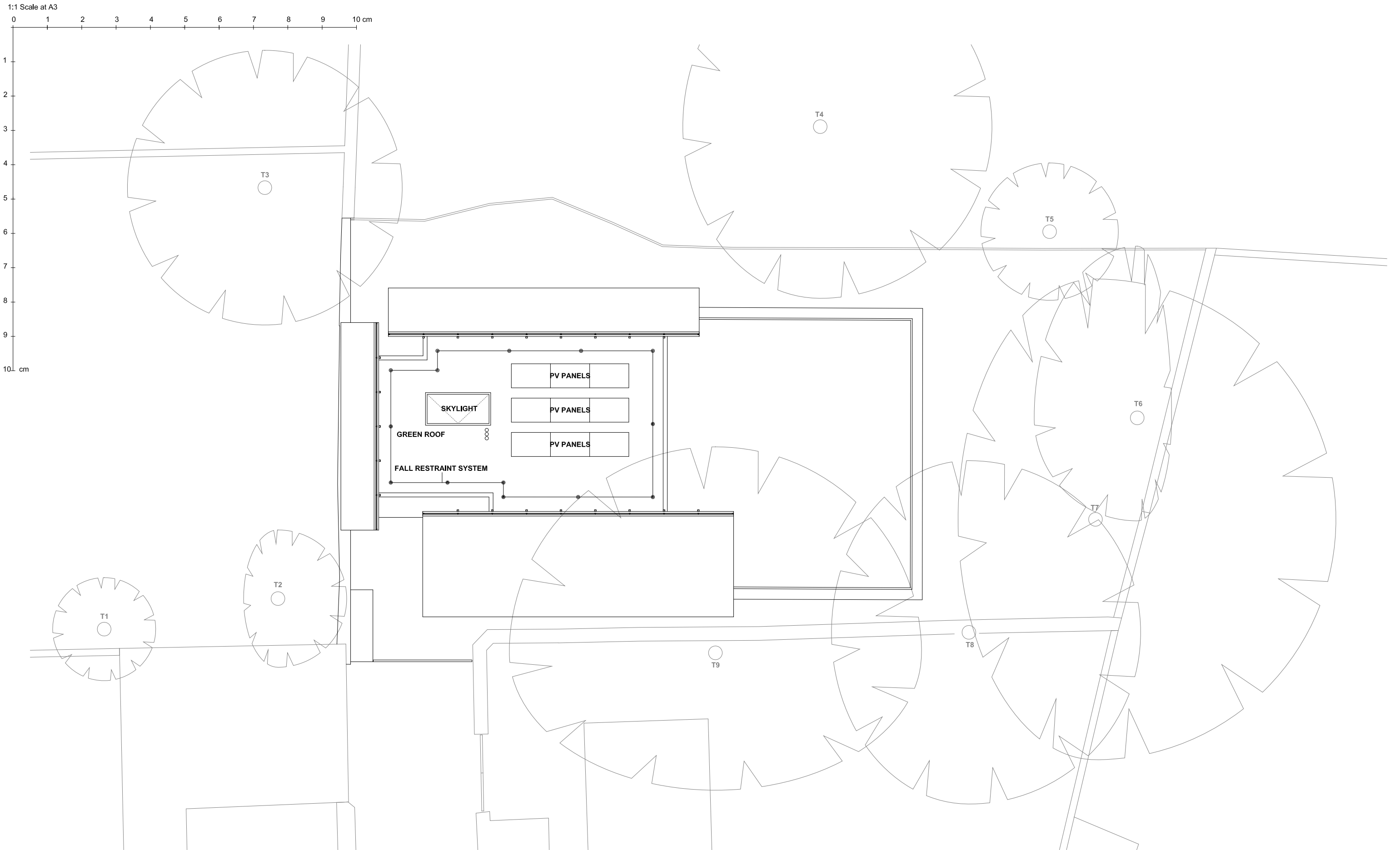
01 Proposed - Roof Plan 1:100 @ A3 / 1:50 @ A1
