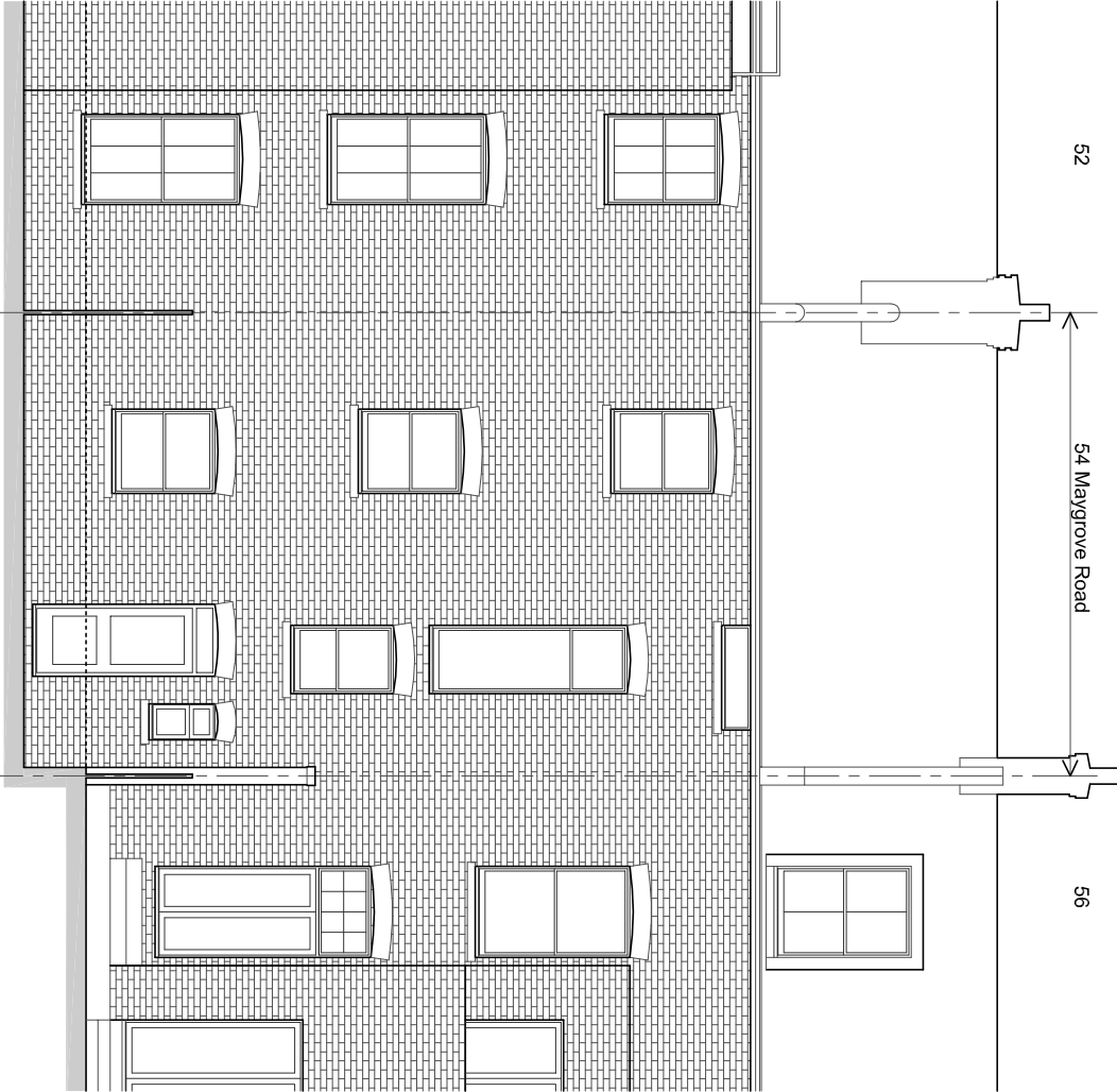
REAR ELEVATION (section B)
