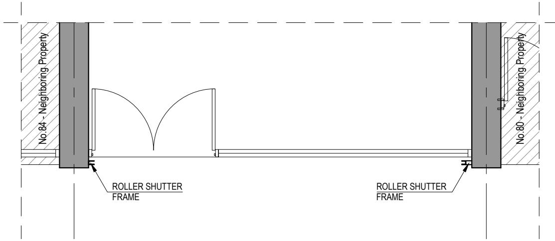
PRE - EXISTING SHOPFRONT - PLAN scale 1:50
