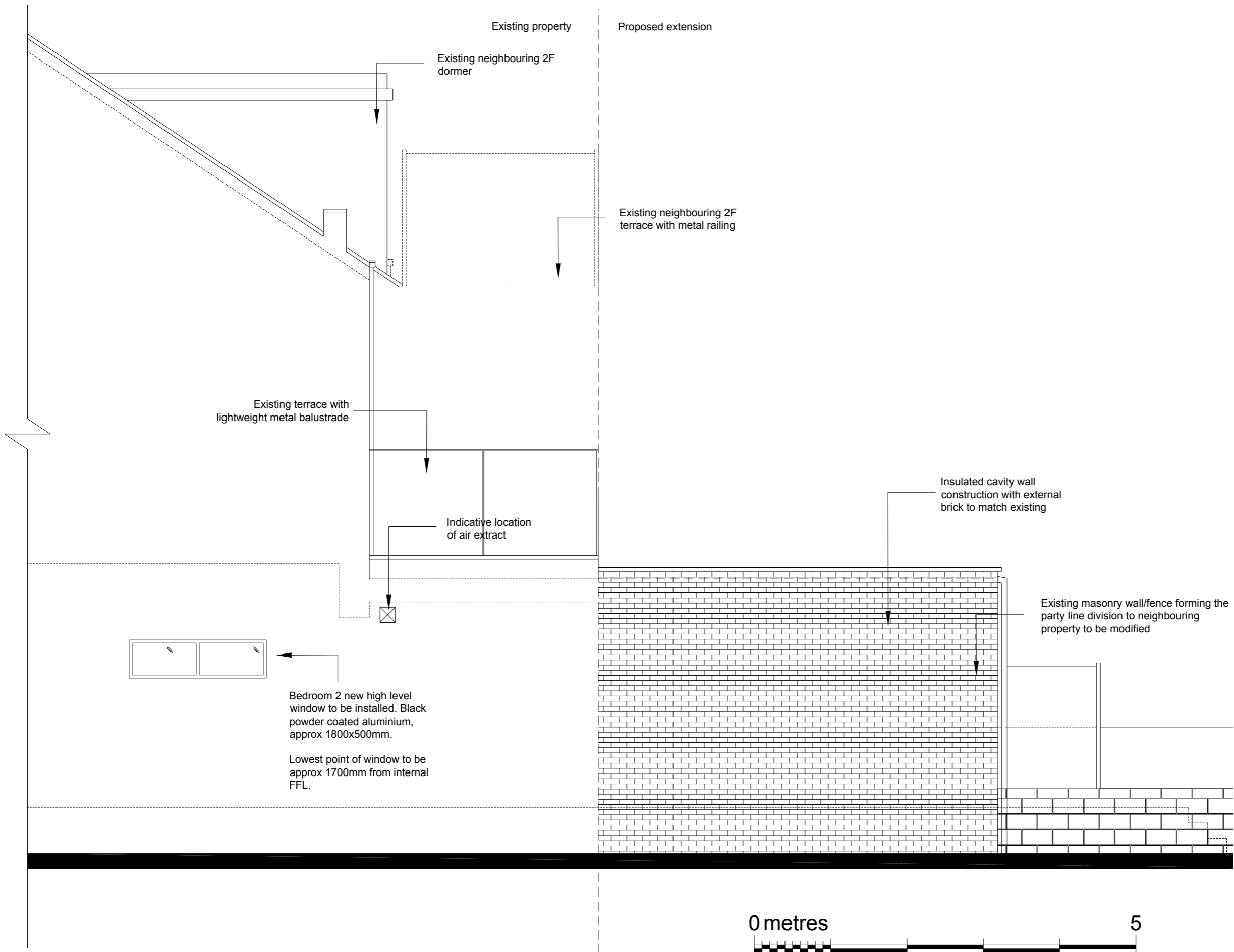
PROPOSED WEST ELEVATION
