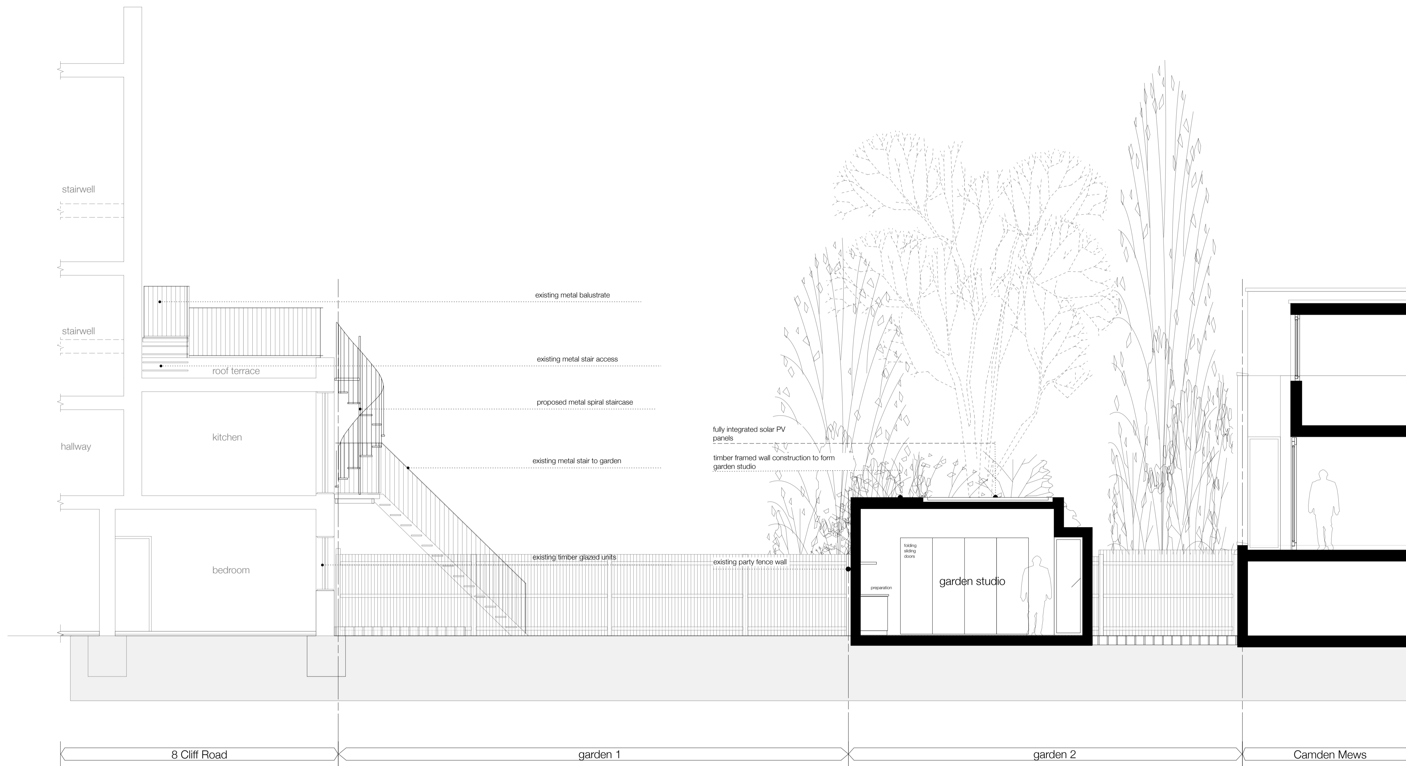
Cross Sectional Elevation of Garden
