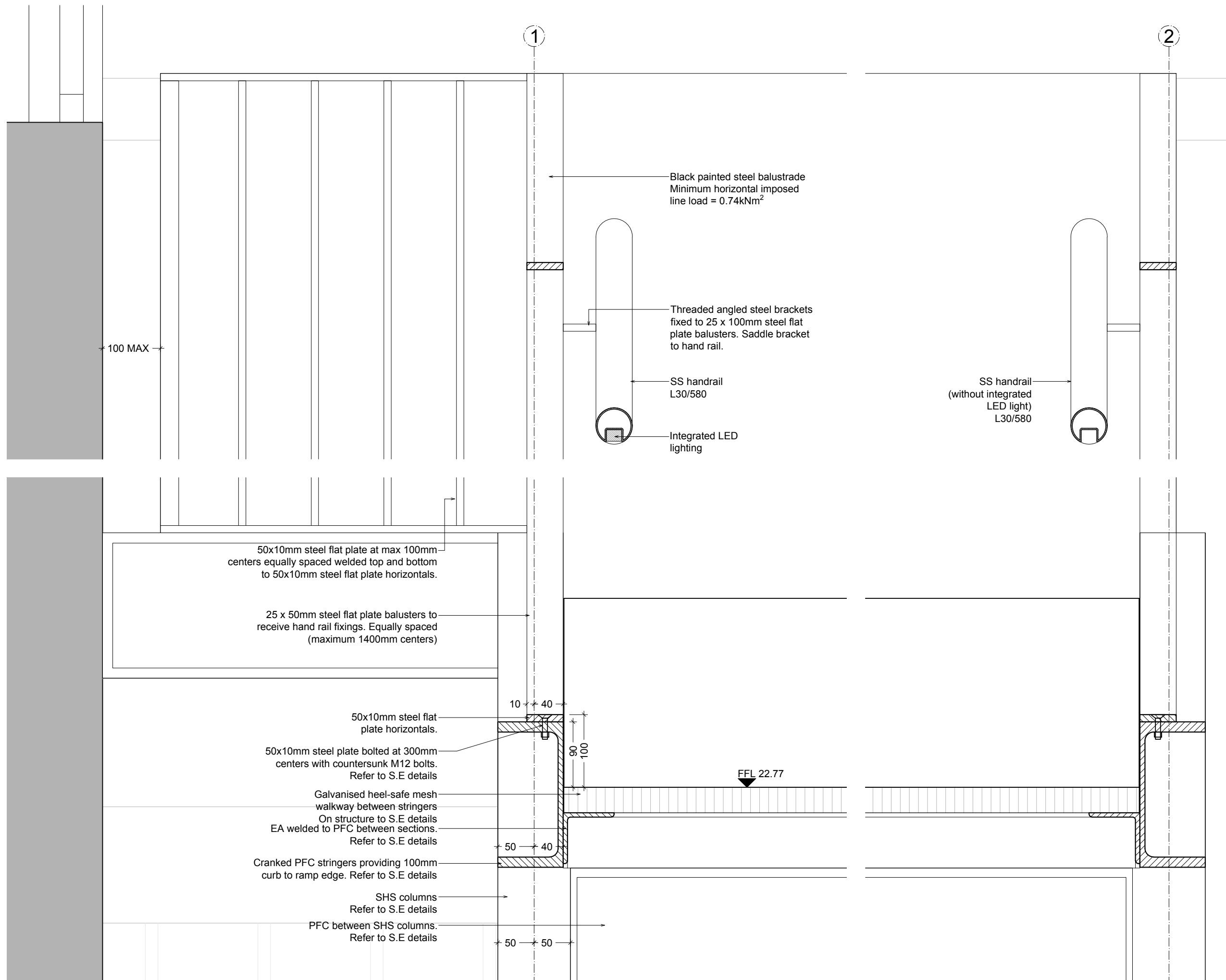
Ramp Stringer and Balustrade
