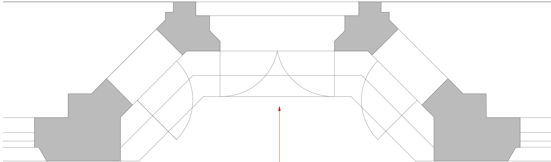
Plan of window steps detail @ 1:25
