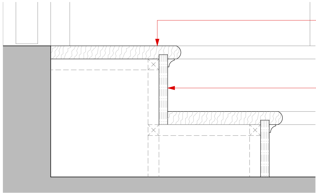
Window steps detail @ 1:5
