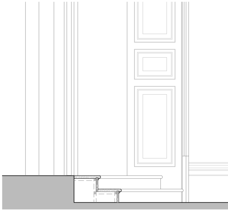
Section /Elevation F window step detail @ 1:25
