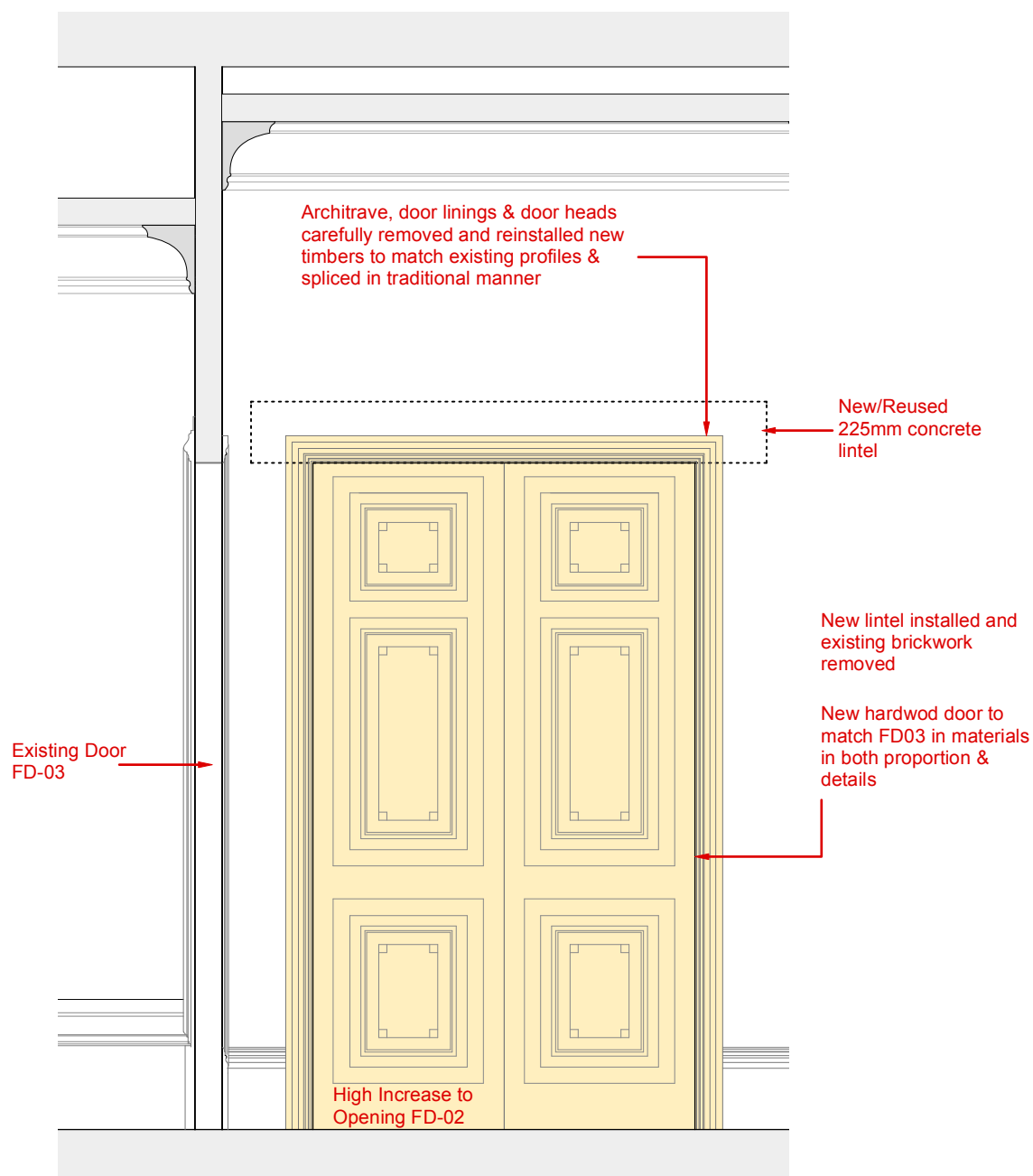
Proposed Elevation E @ 1:25
