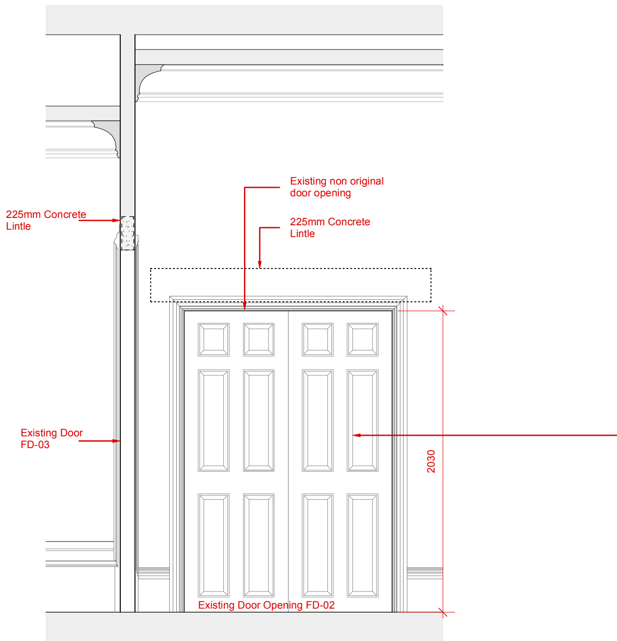
Existing Elevation E @ 1:25
