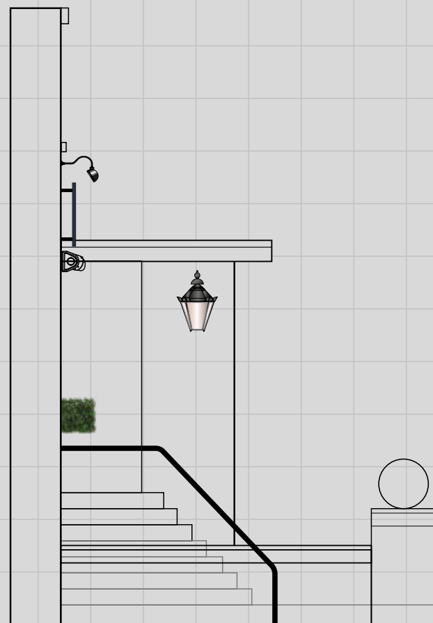
SIDE ELEVATION AWNING CLOSED
