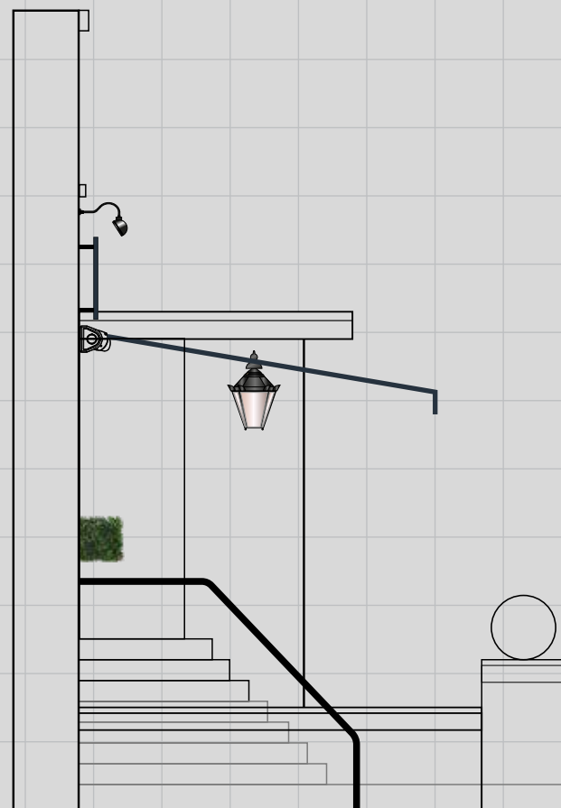
SIDE ELEVATION AWNING OPEN
