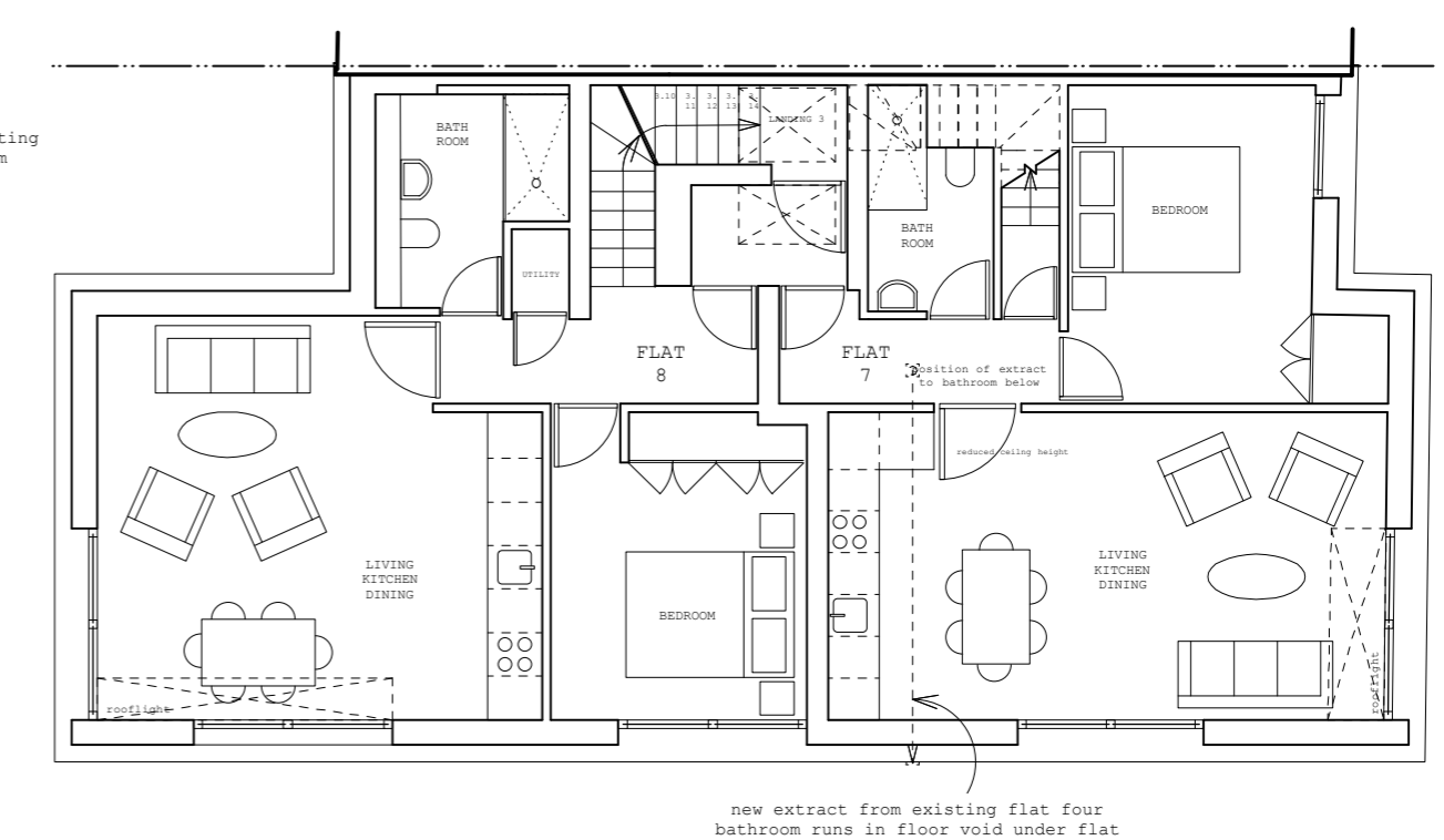
04 4F Plan
