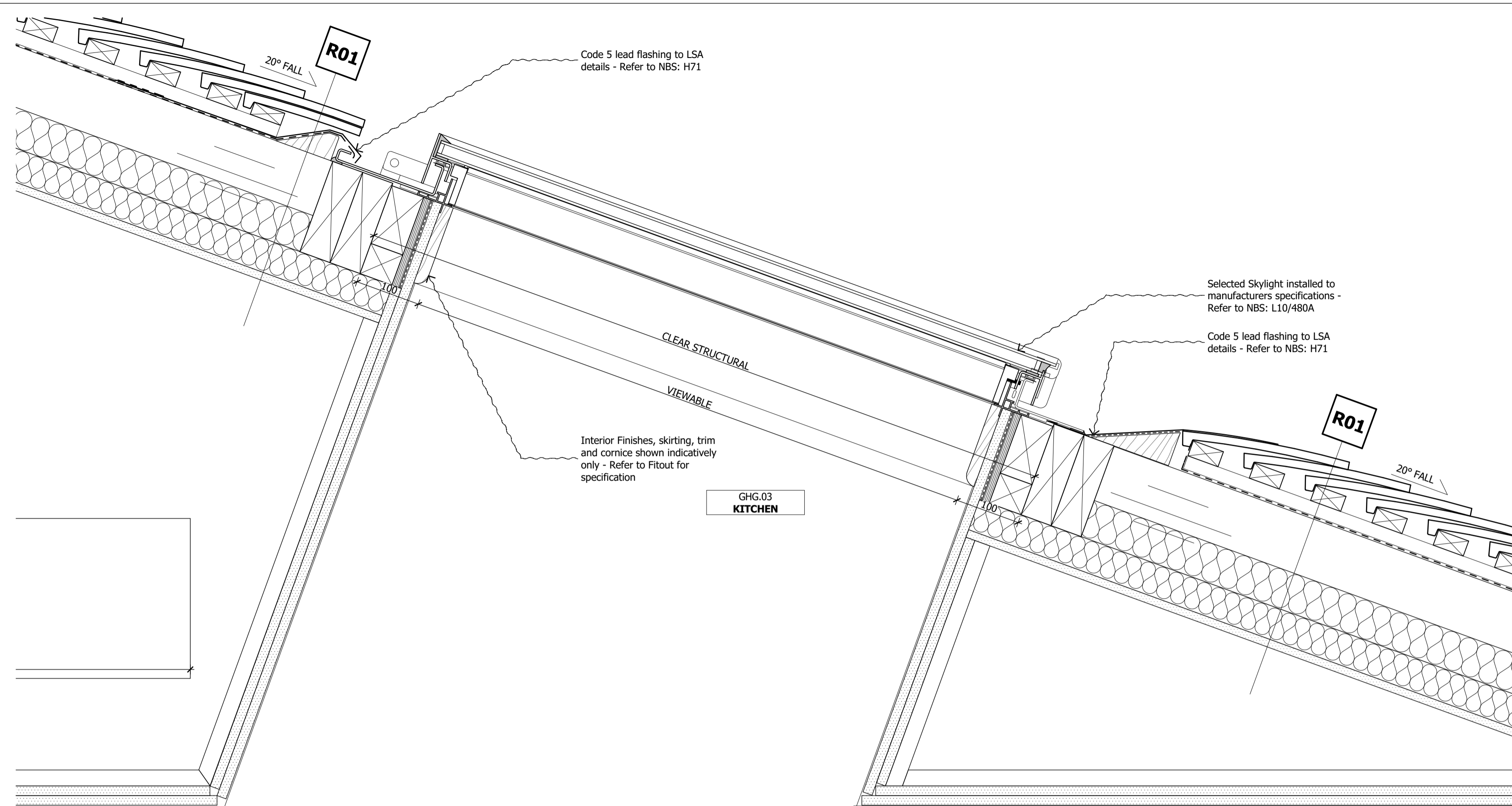
3 SCALE 1:5 @ A1, 1:10 @ A3 SECTION B-B DETAIL - NEW EXTENSION - SKYLIGHT
