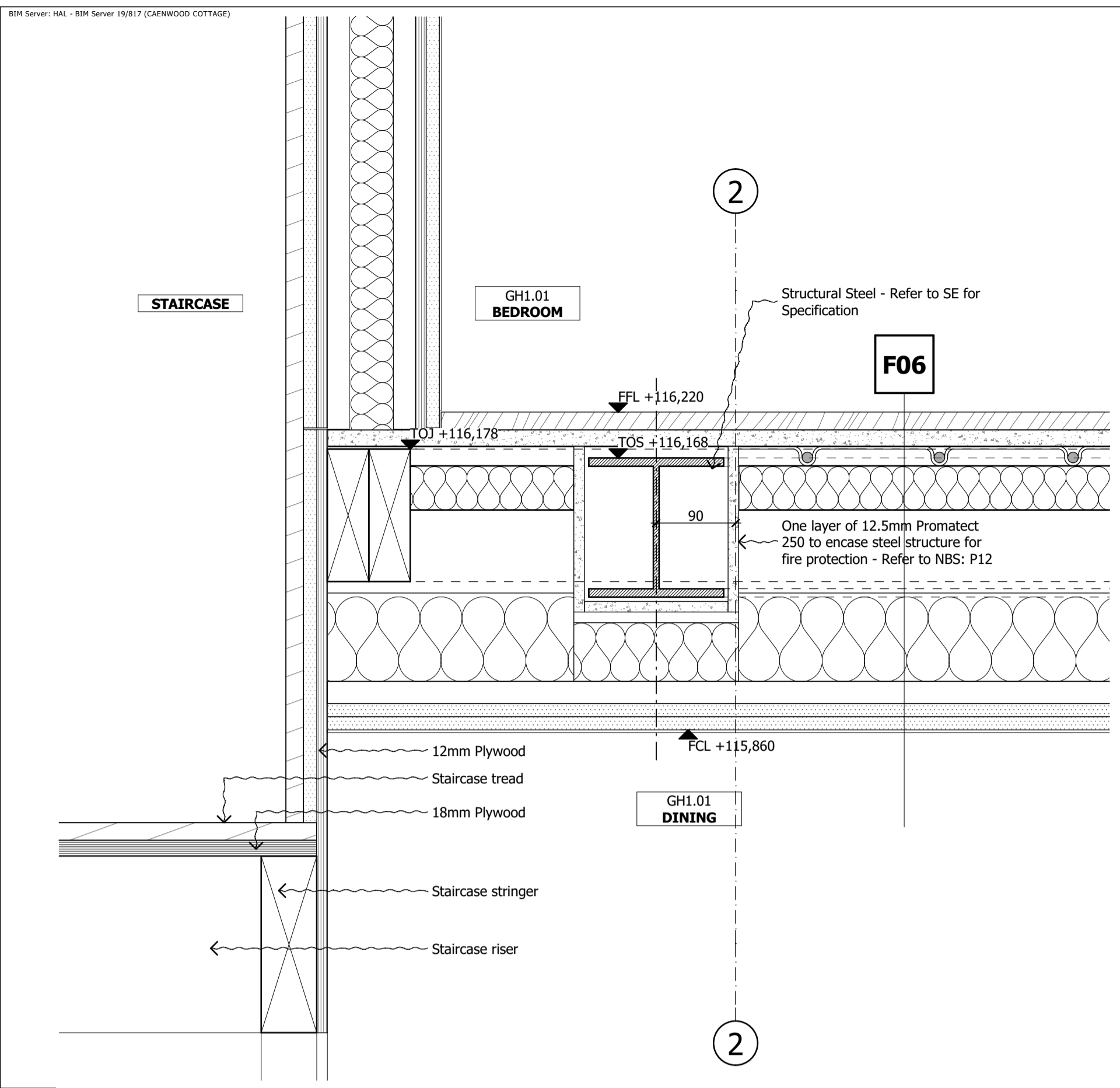
1 SCALE 1:5 @ A1, 1:10 @ A3 SECTION C-C DETAIL - FIRST FLOOR TO STAIR
