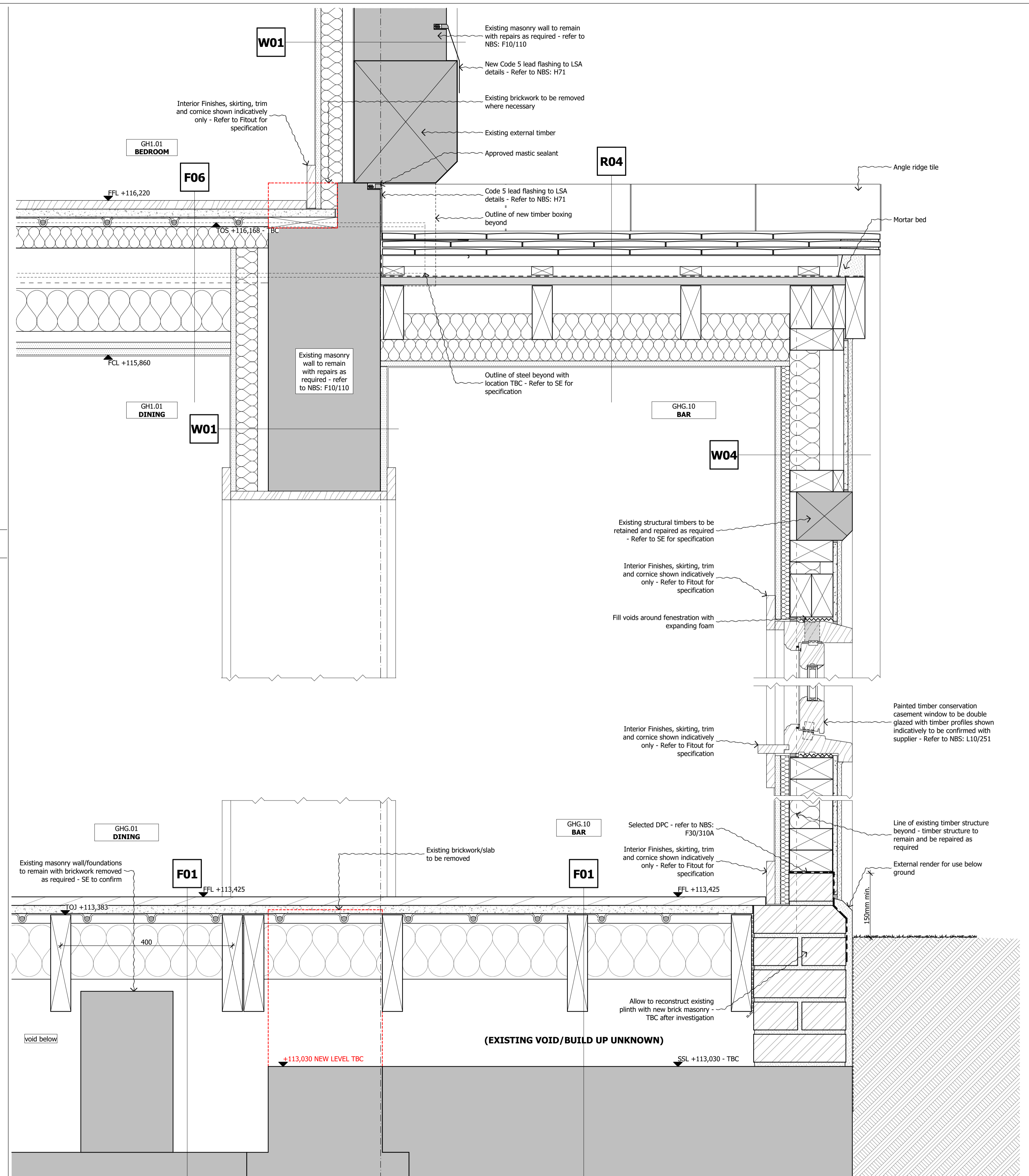
3 SCALE 1:5 @ A1, 1:10 @ A3 SECTION C-C DETAIL - BAR (GHG.10) BELOW GROUND, FENESTRATION & ROOF TO FIRST FLOOR INTERSECTION
