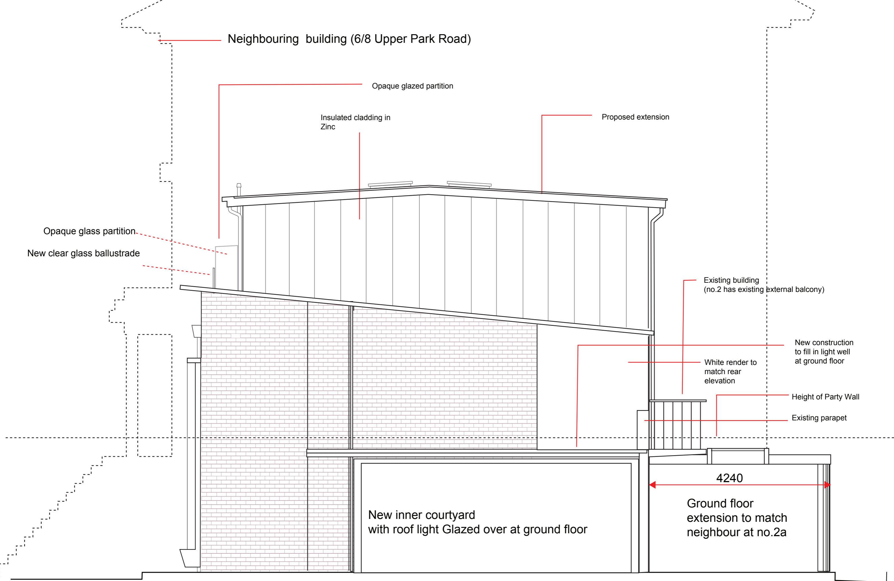
(West) End Elevation of Terrace 2-4b Upper Park Road
