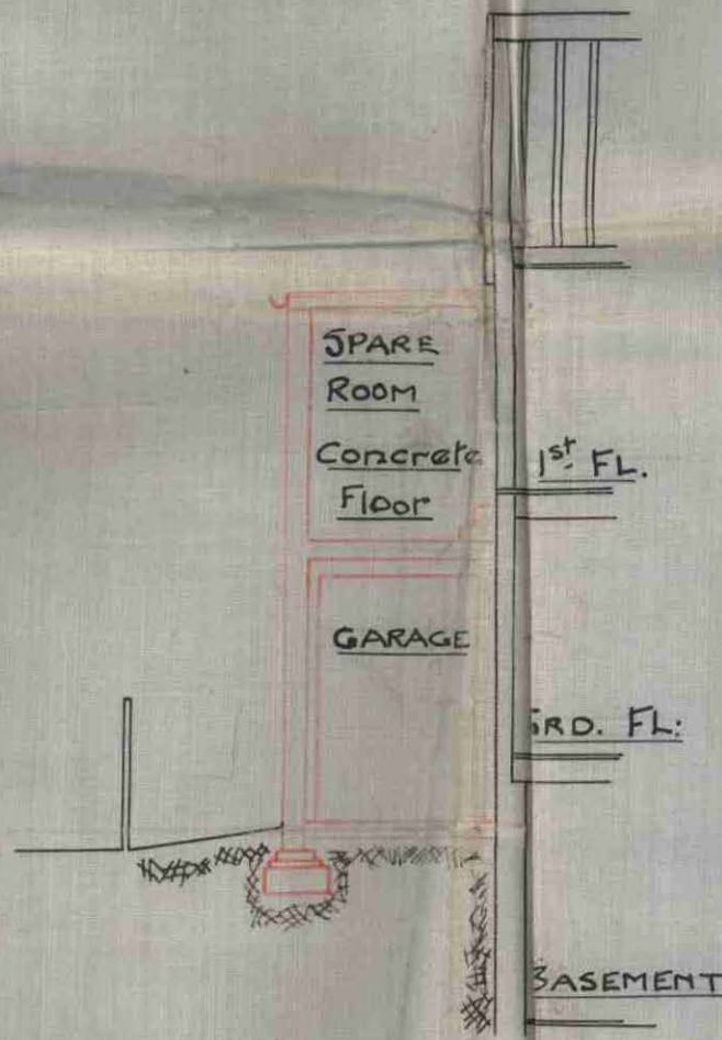
SECTION B-B.
