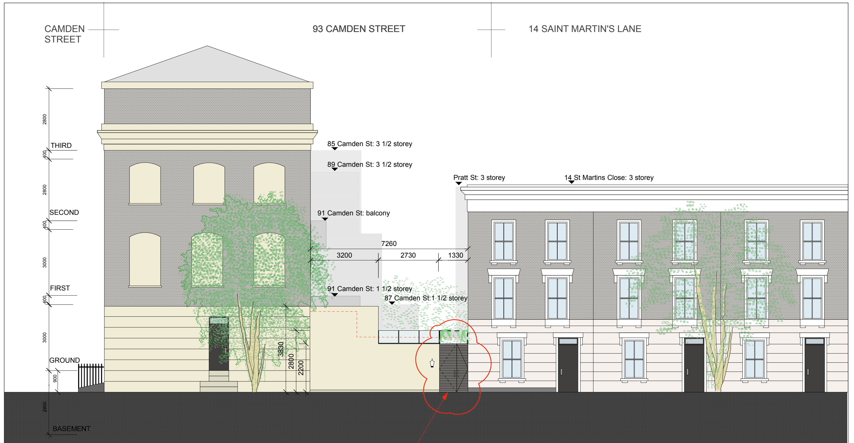
(A/2.21) PROPOSED NORTH ELEVATION: SAINT MARTIN'S LANE scale 1:100
