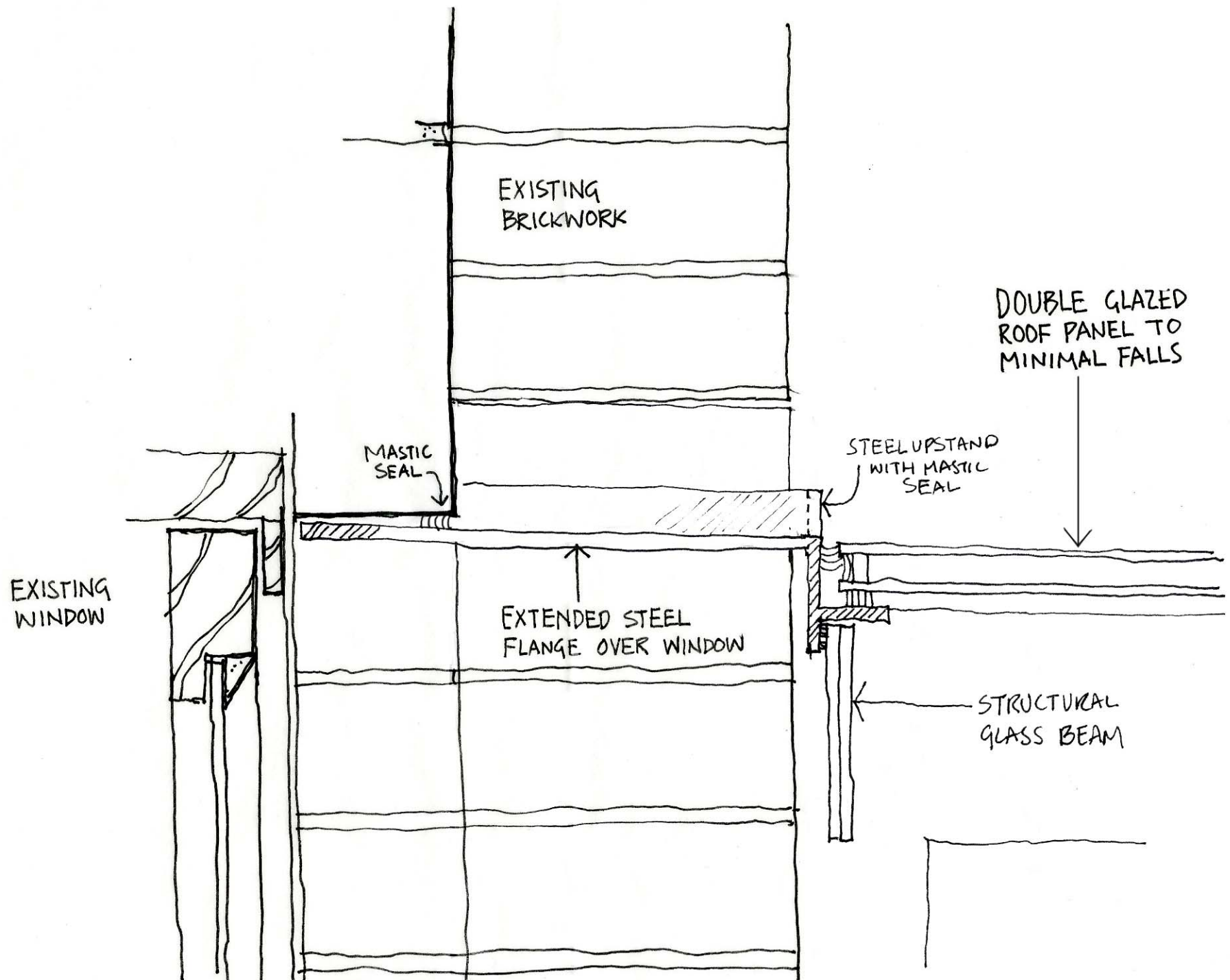
DETAIL 1-REV.A ROOF CONNECTION AT WINDOW HEAD
