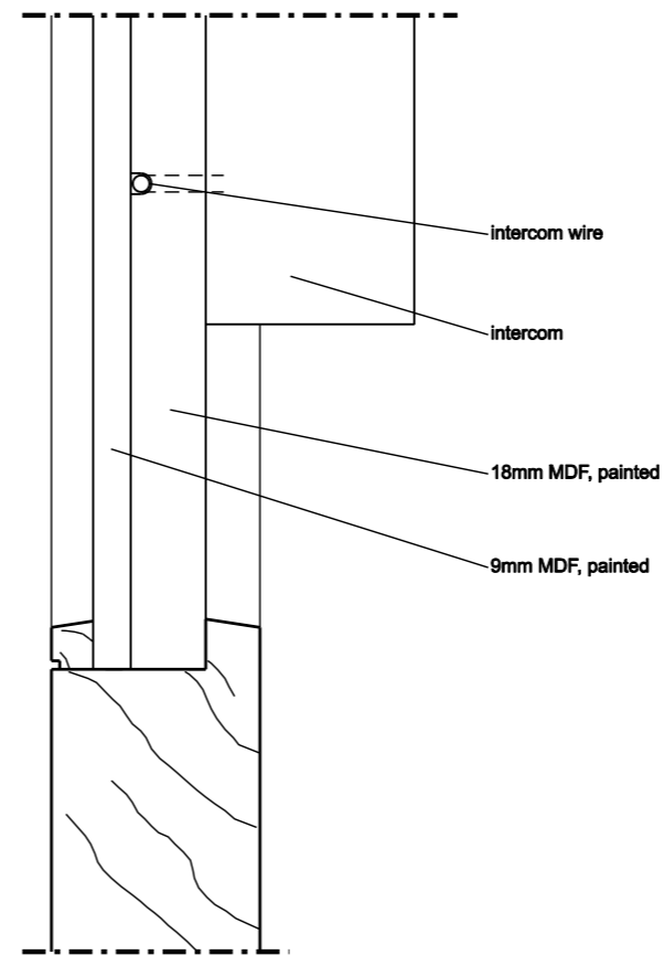
Section through Fixed Panel
