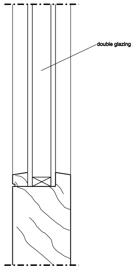
Section through Glazed Door
