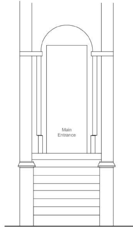
Existing elevation Scale 1:50
