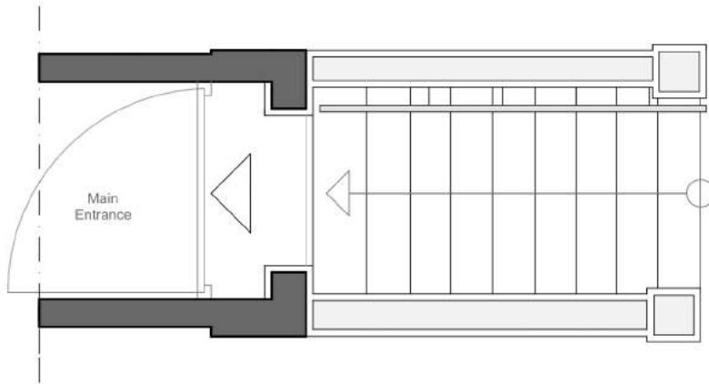
Proposed plan Scale 1:50
