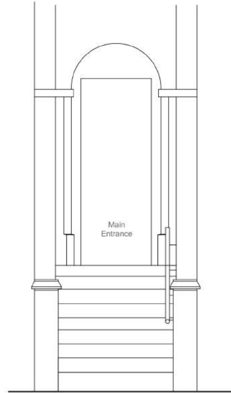
Proposed elevation Scale 1:50
