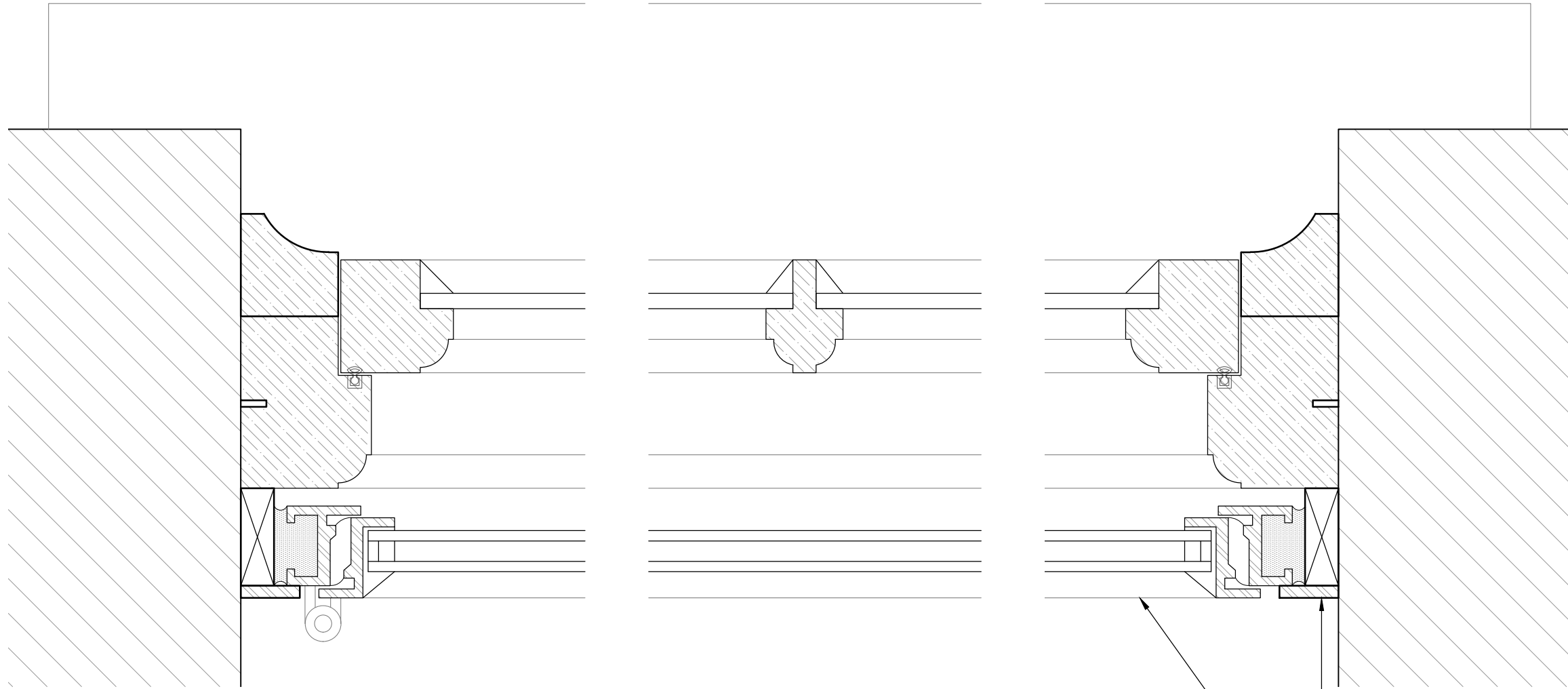
Plan Details
