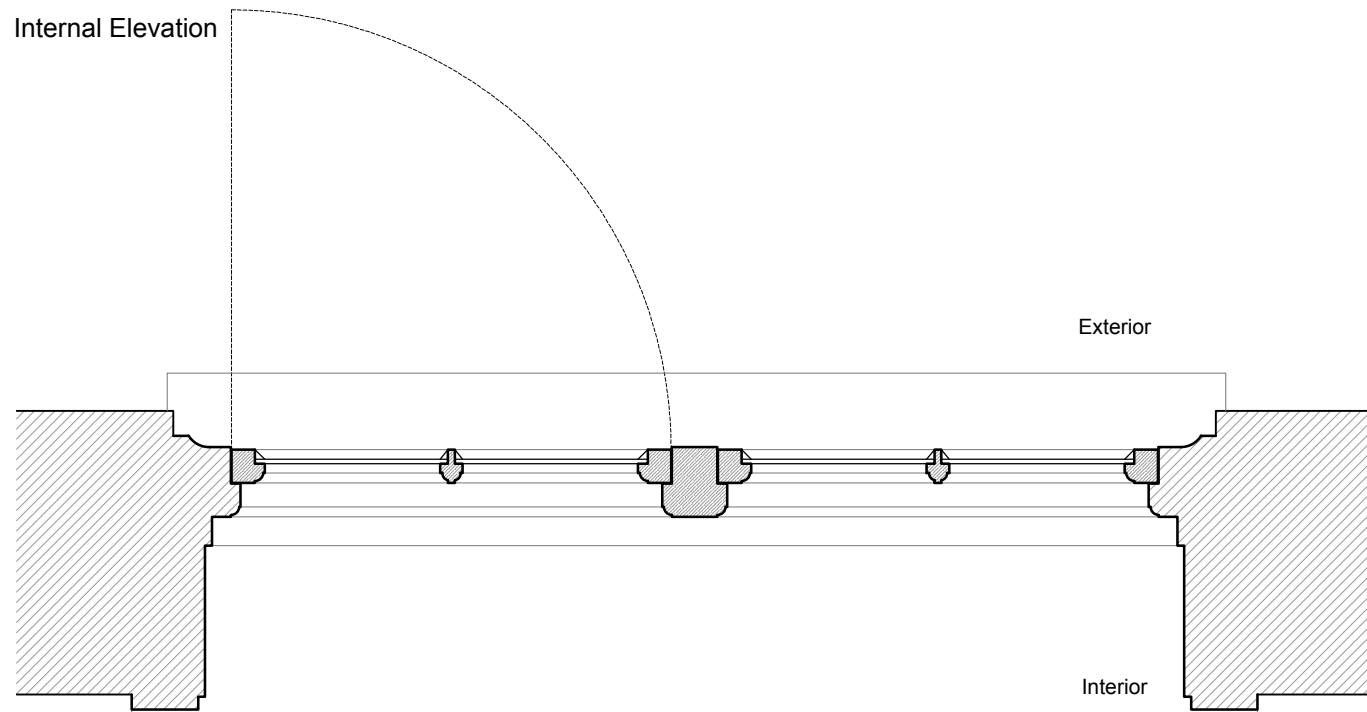
Detail Plan
