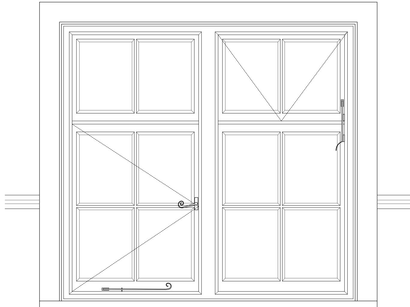
Internal Elevation
