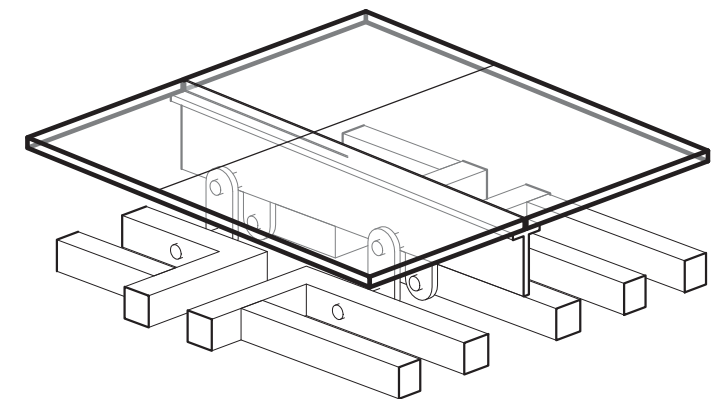
③ Terrace Structure detail 3D
