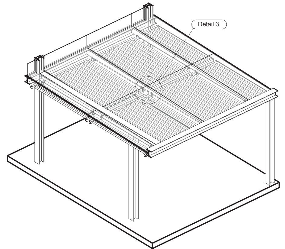
② Terrace Structure detail Section 3D
