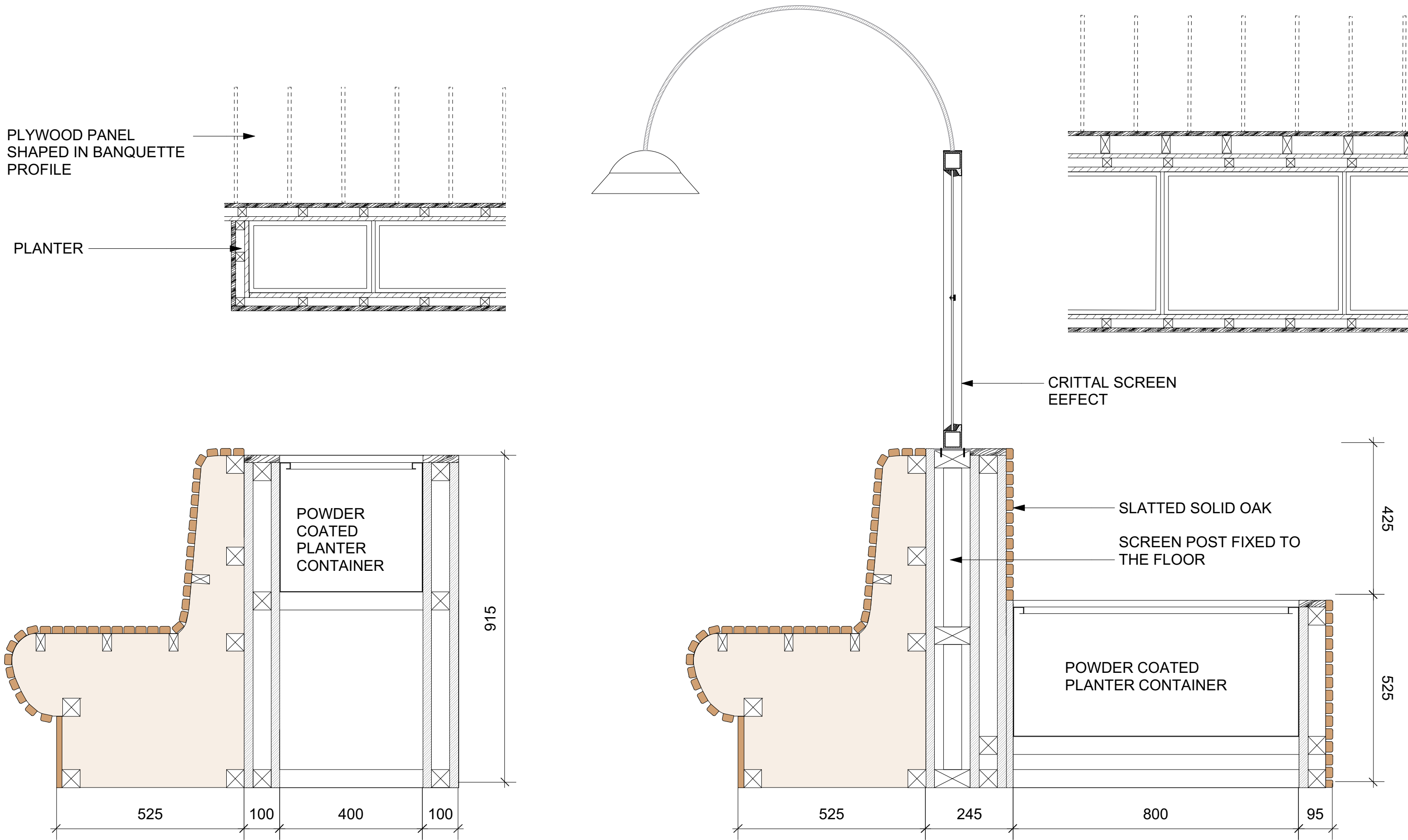
Type A Banquette: 400 mm wide planter, without crittall screen against the wall facade
