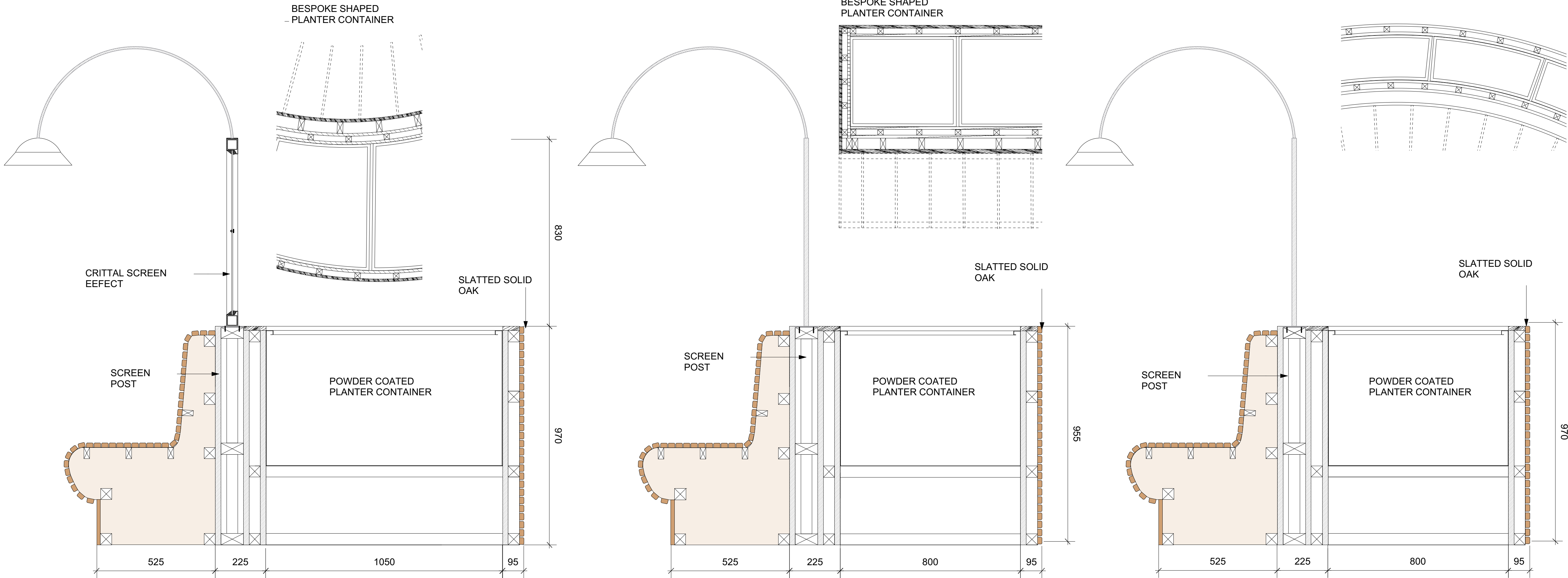
Type E Banquette: 400 mm wide planter, on curve
