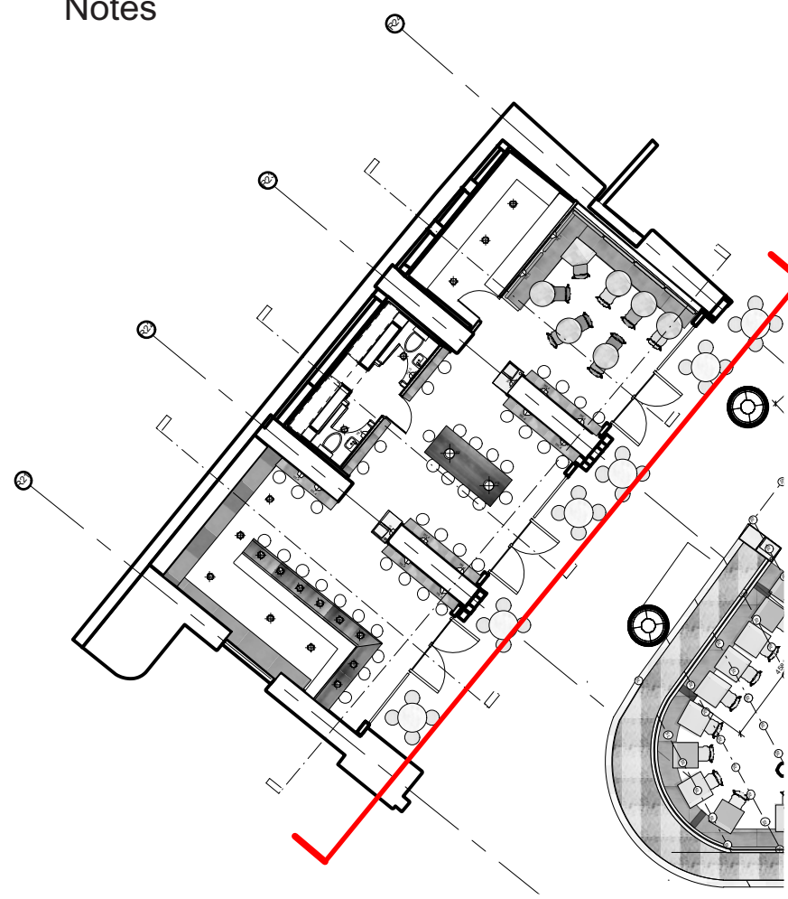
GROUND LEVEL PLAN 1:200
