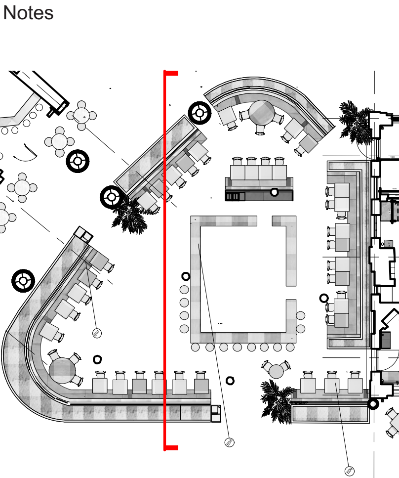
GROUND LEVEL PLAN 1:200
