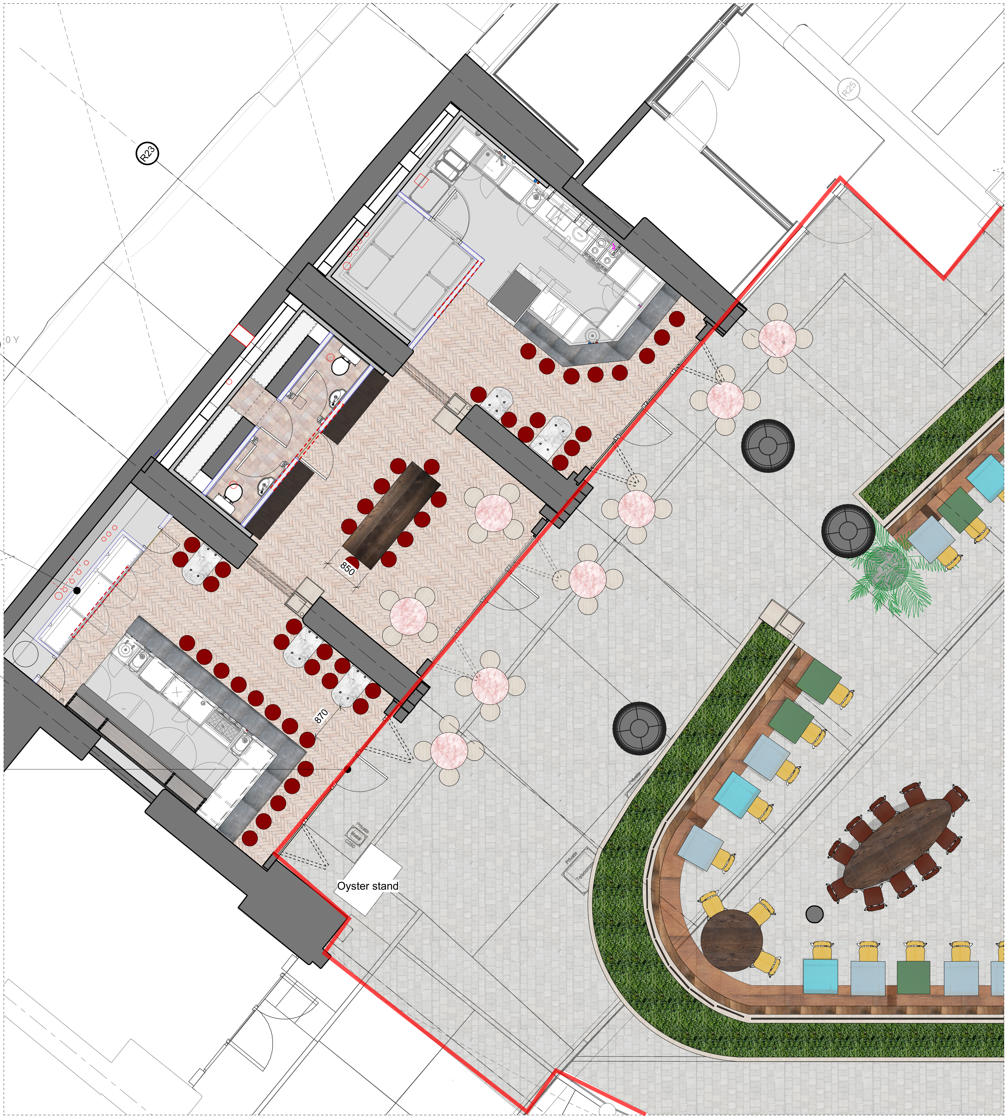
1 Proposed External Yard Level Floor Plan 1:50
