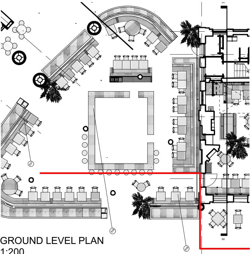
GROUND LEVEL PLAN 1:200
