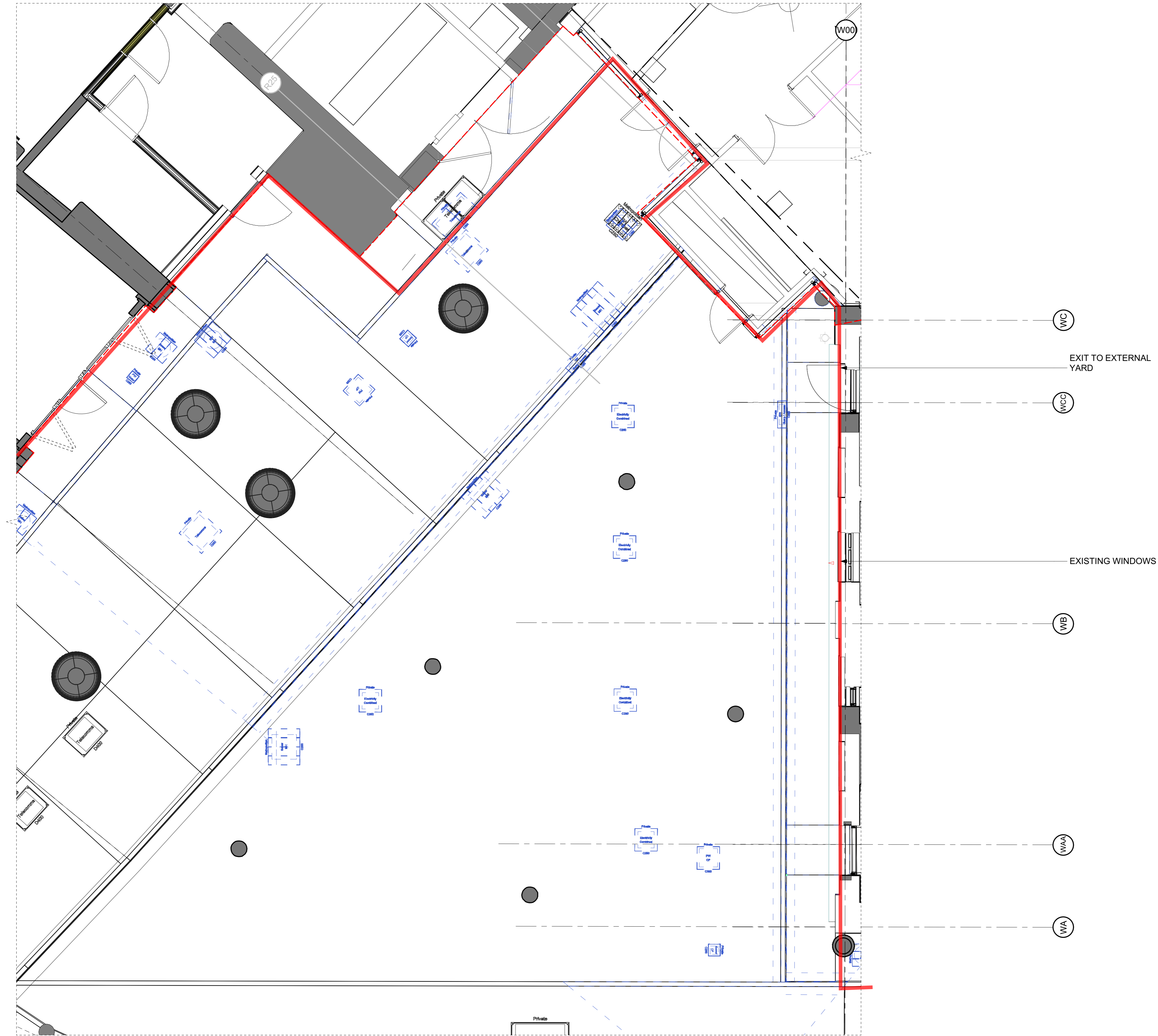
1 Existing External Yard Level Floor Plan 1:50
