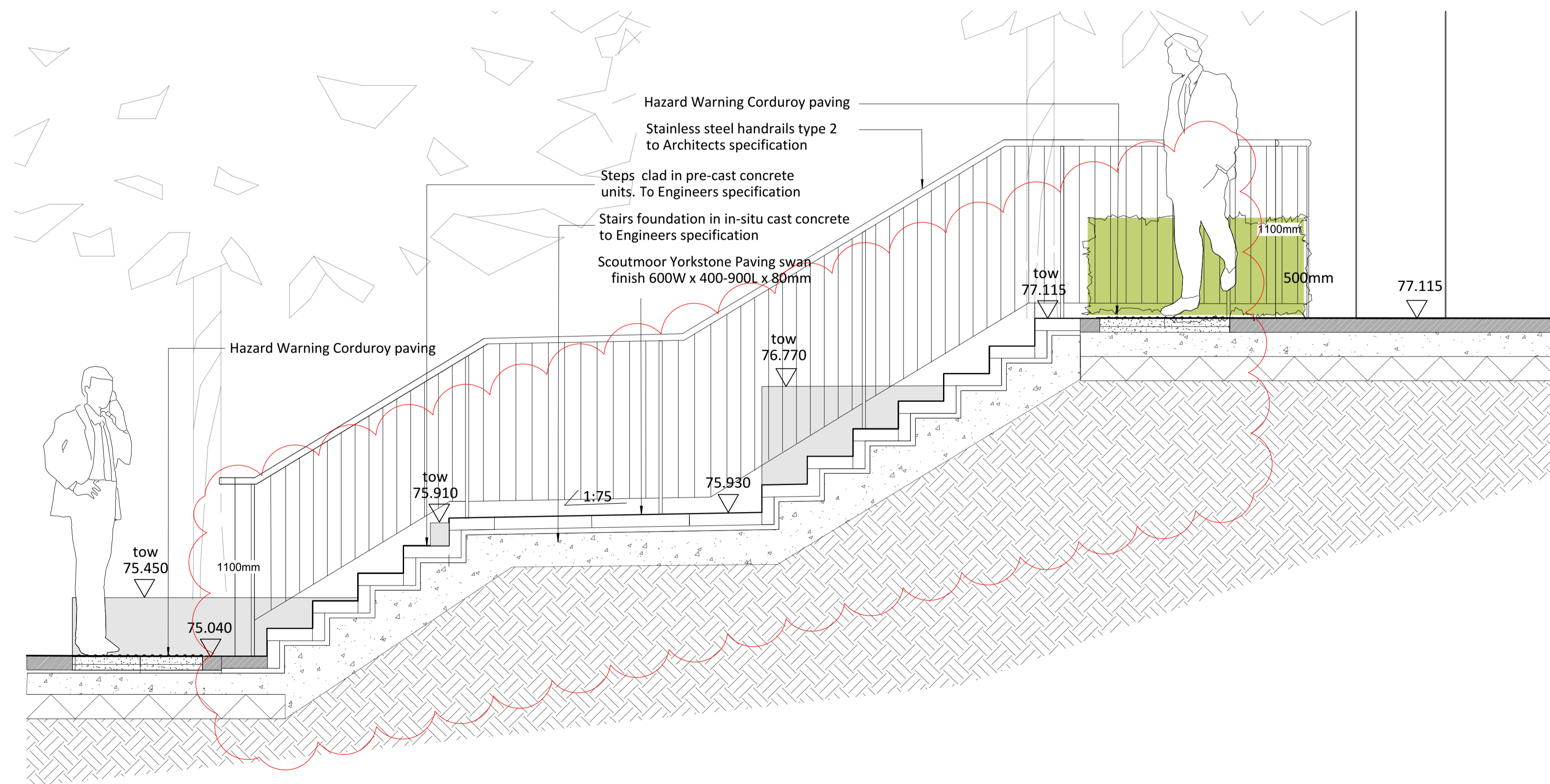
F - SECTIONAL ELEVATION 1:20
