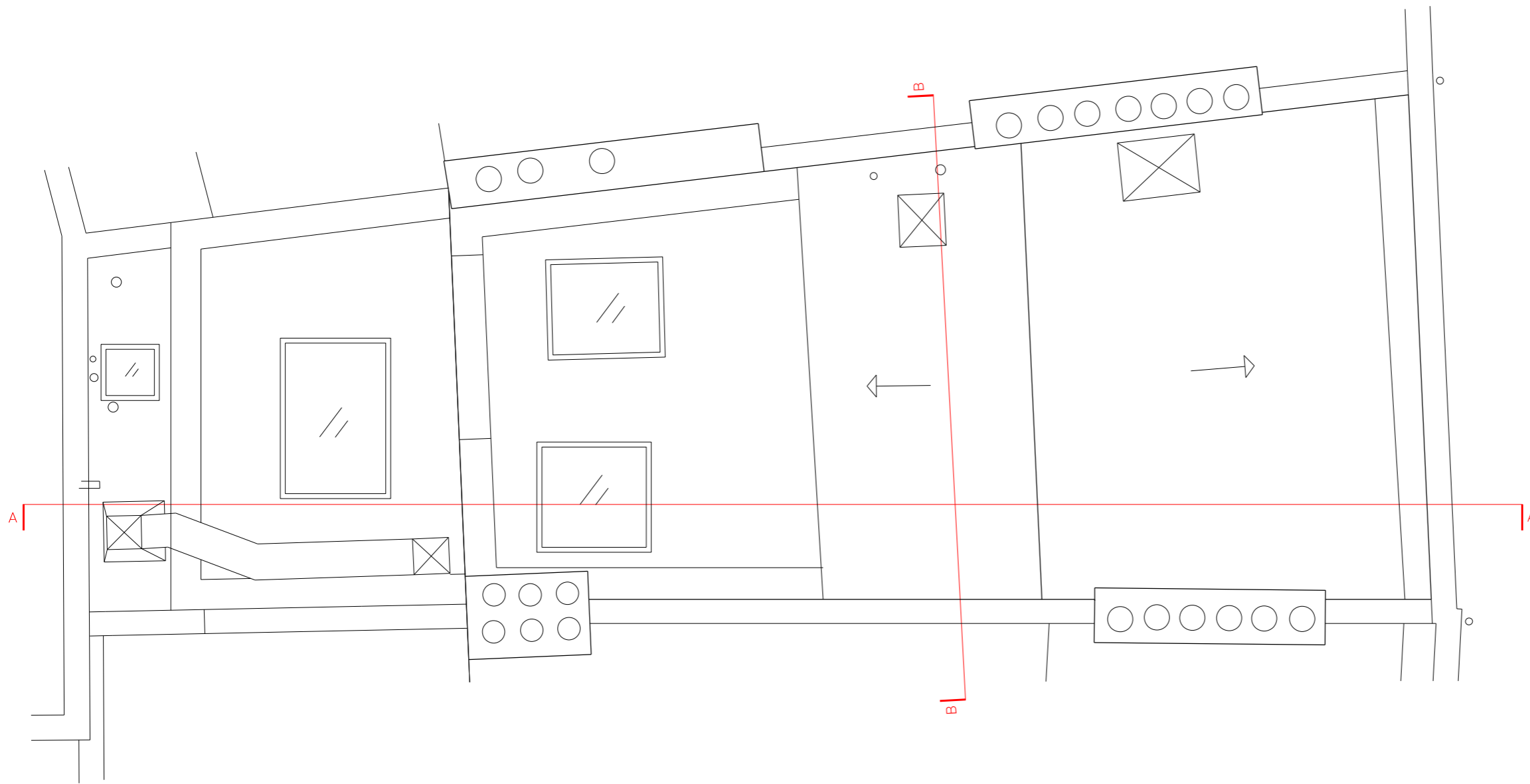
01 PLAN - PROPOSED ROOF PLAN SCALE 1:50
