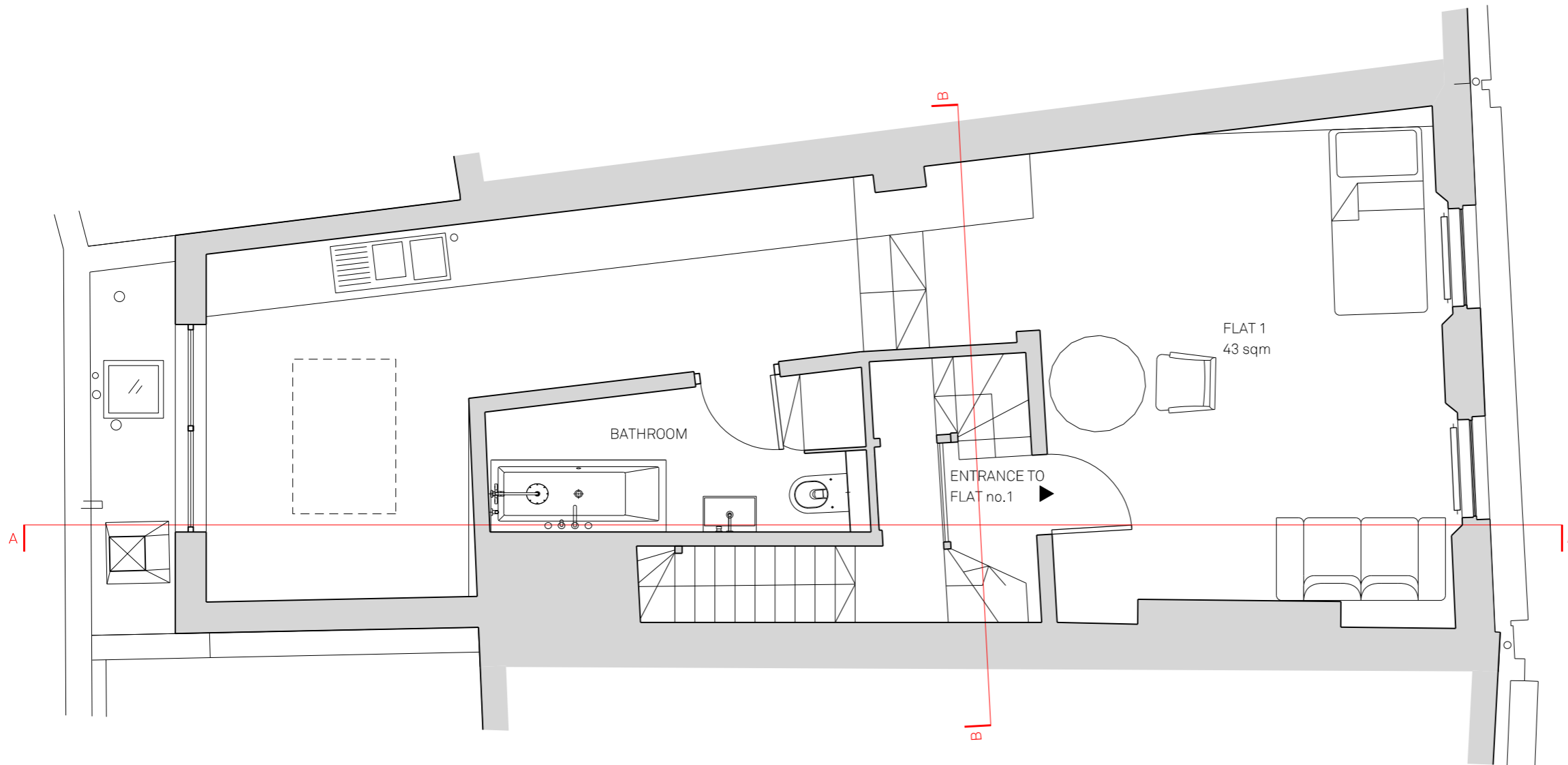
01 PLAN - PROPOSED FIRST FLOOR SCALE 1:50
