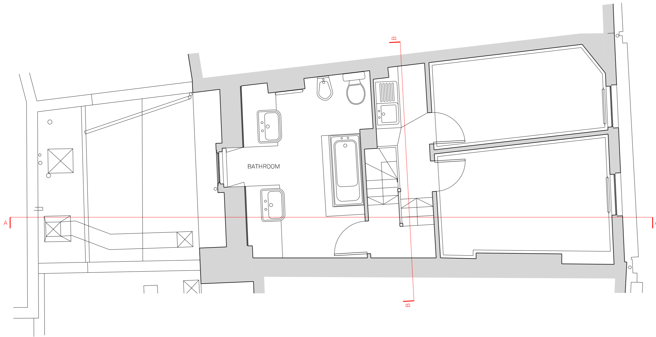
01 PLAN - EXISTING THIRD FLOOR SCALE 1:50
