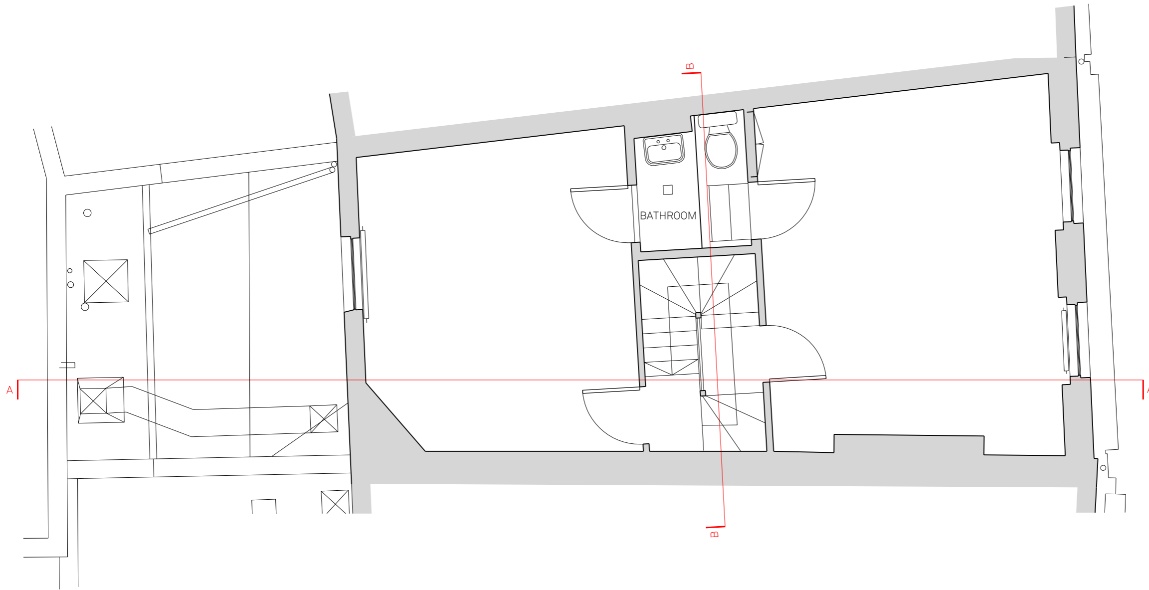
01 PLAN - EXISTING SECOND FLOOR SCALE 1:50
