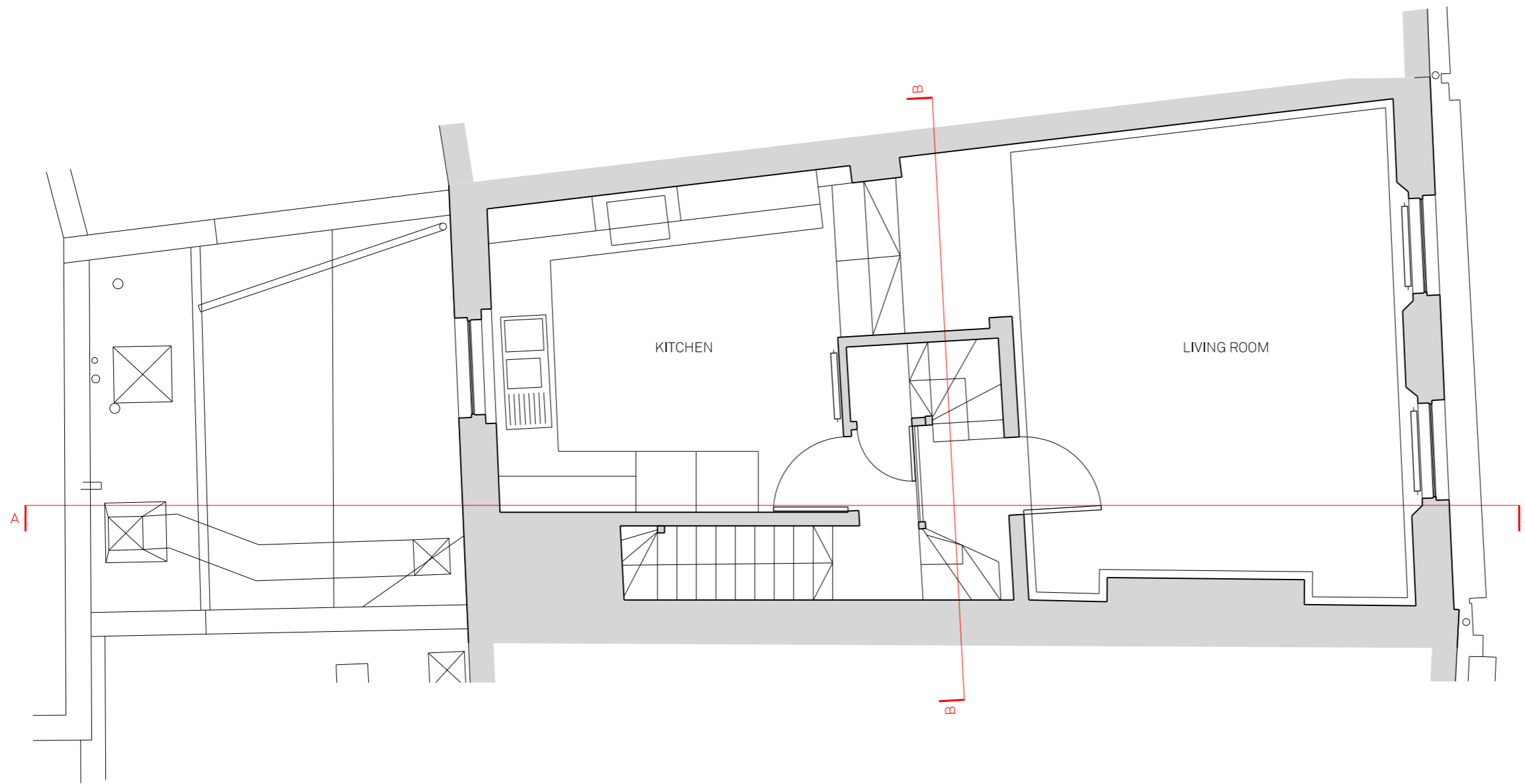
01 PLAN - EXISTING FIRST FLOOR SCALE 1:50
