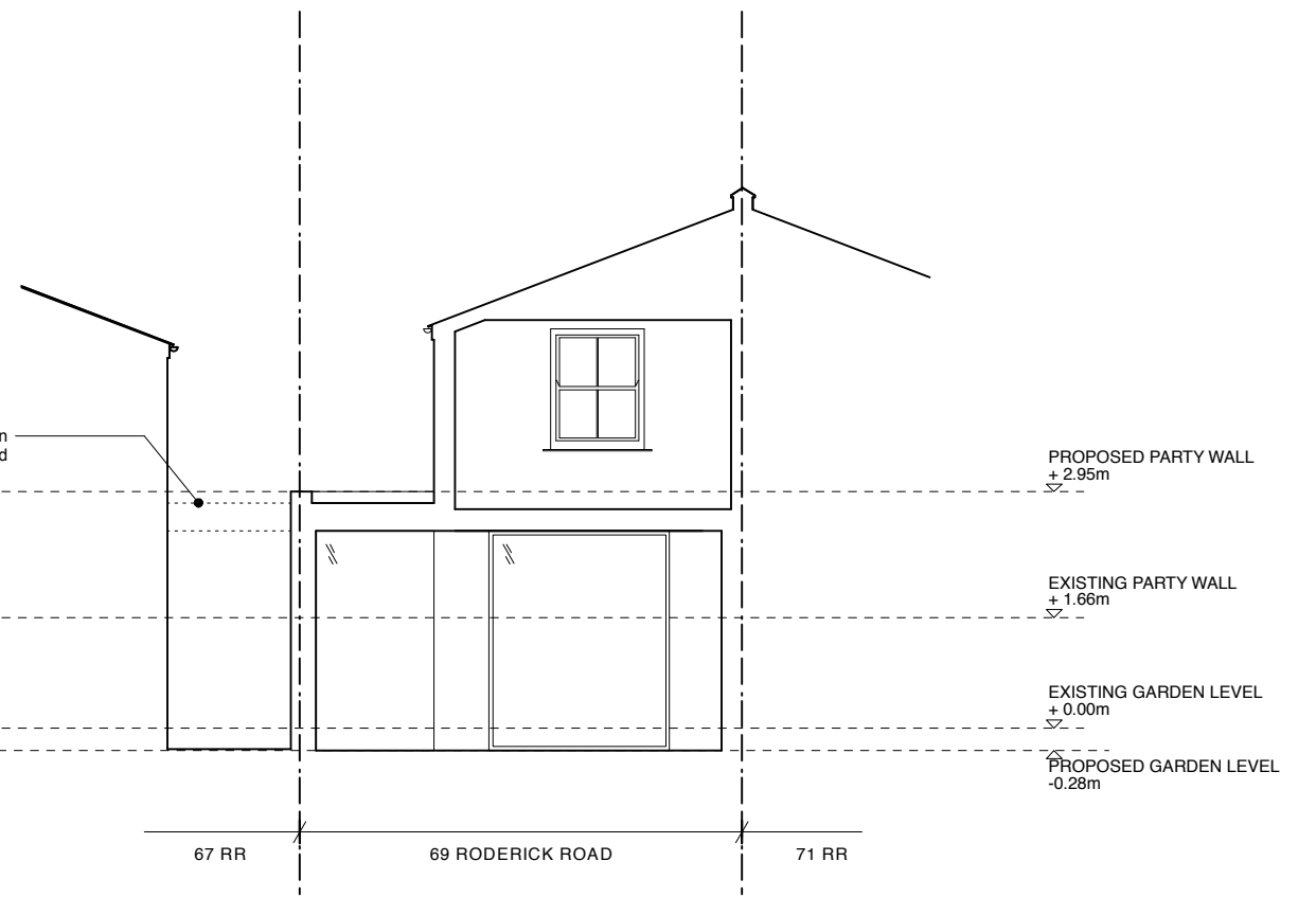
SECTION AA AS PROPOSED
