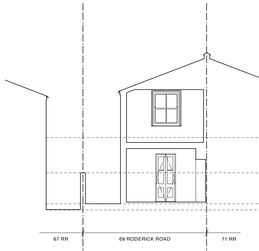
SECTION AA AS EXISTING
