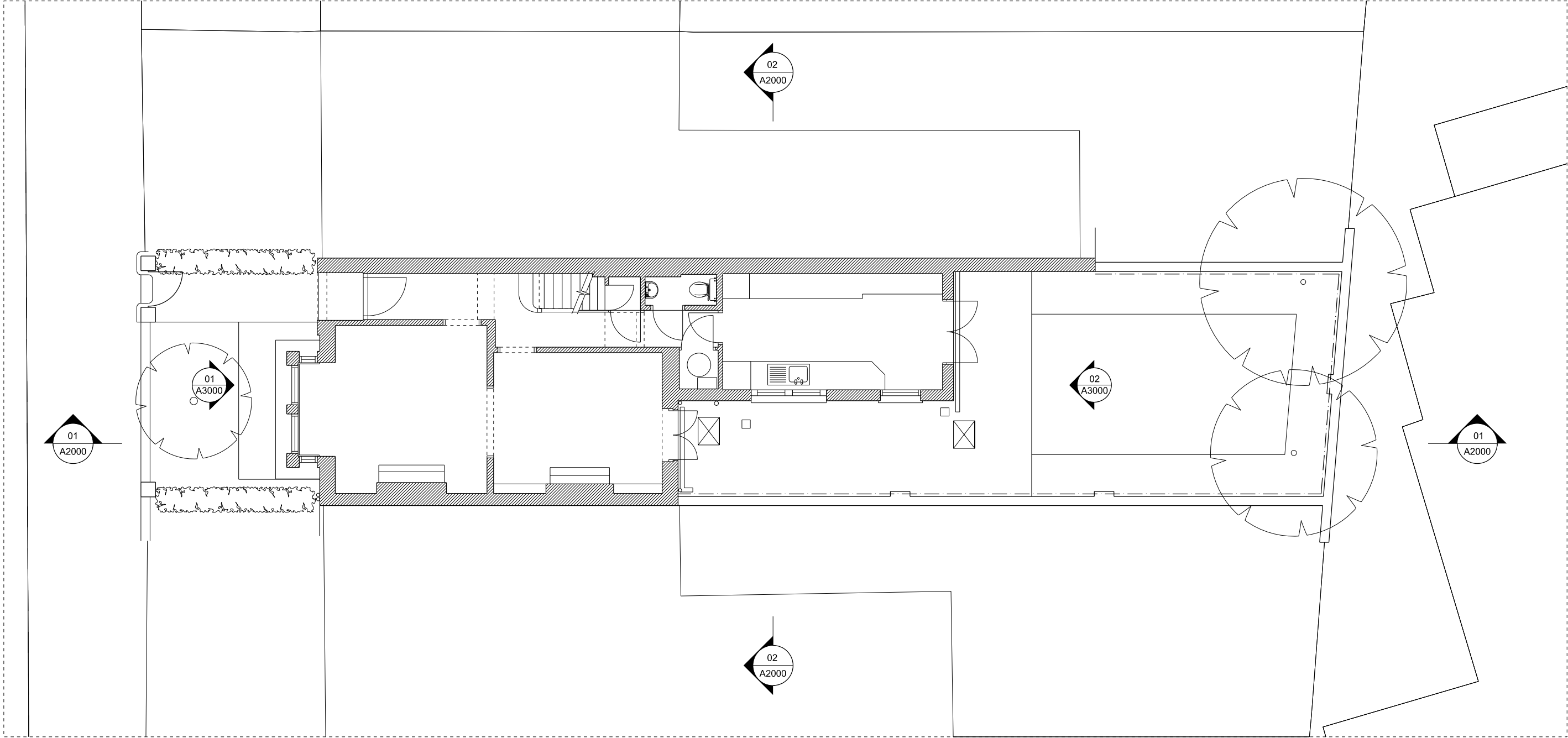
01 EXISTING GROUND FLOOR PLAN A1000 1:100 @ A3
