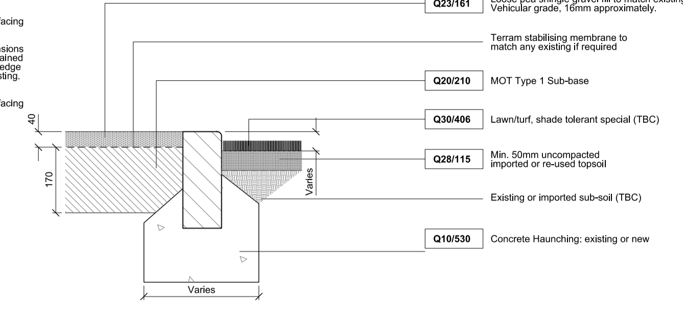
Granite Kerb/Edge Detail 1
