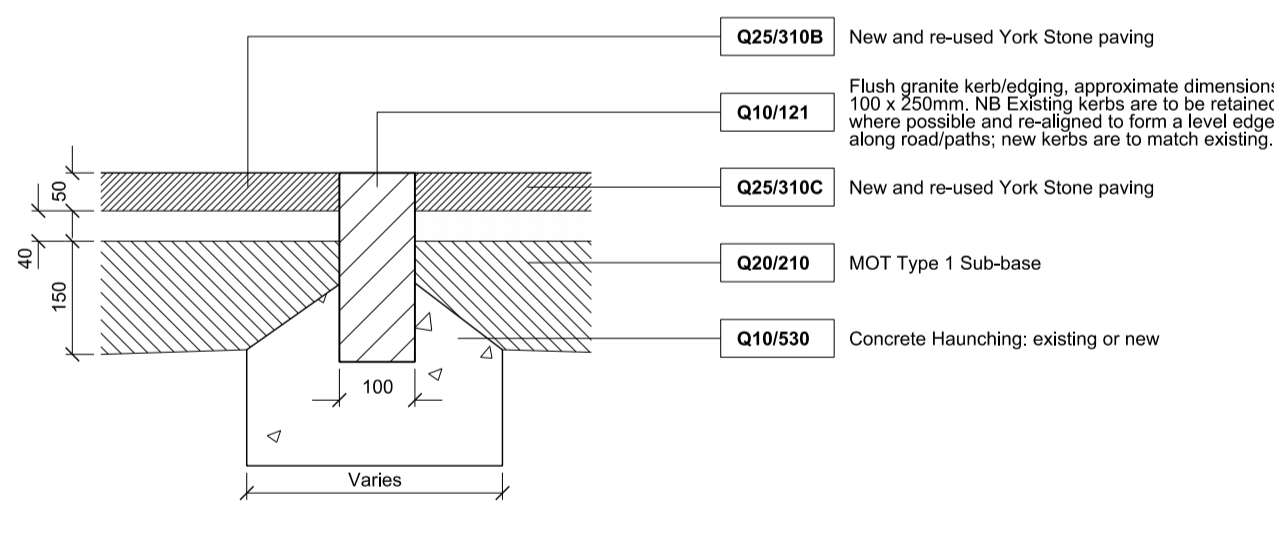
Granite Edge & York Stone Threshold Detail
