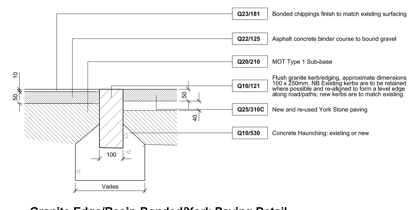
Granite Edge/Resin-Bonded/York Paving Detail
