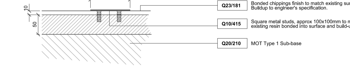
Disabled parking bay metal stud demarcation (1:5)
