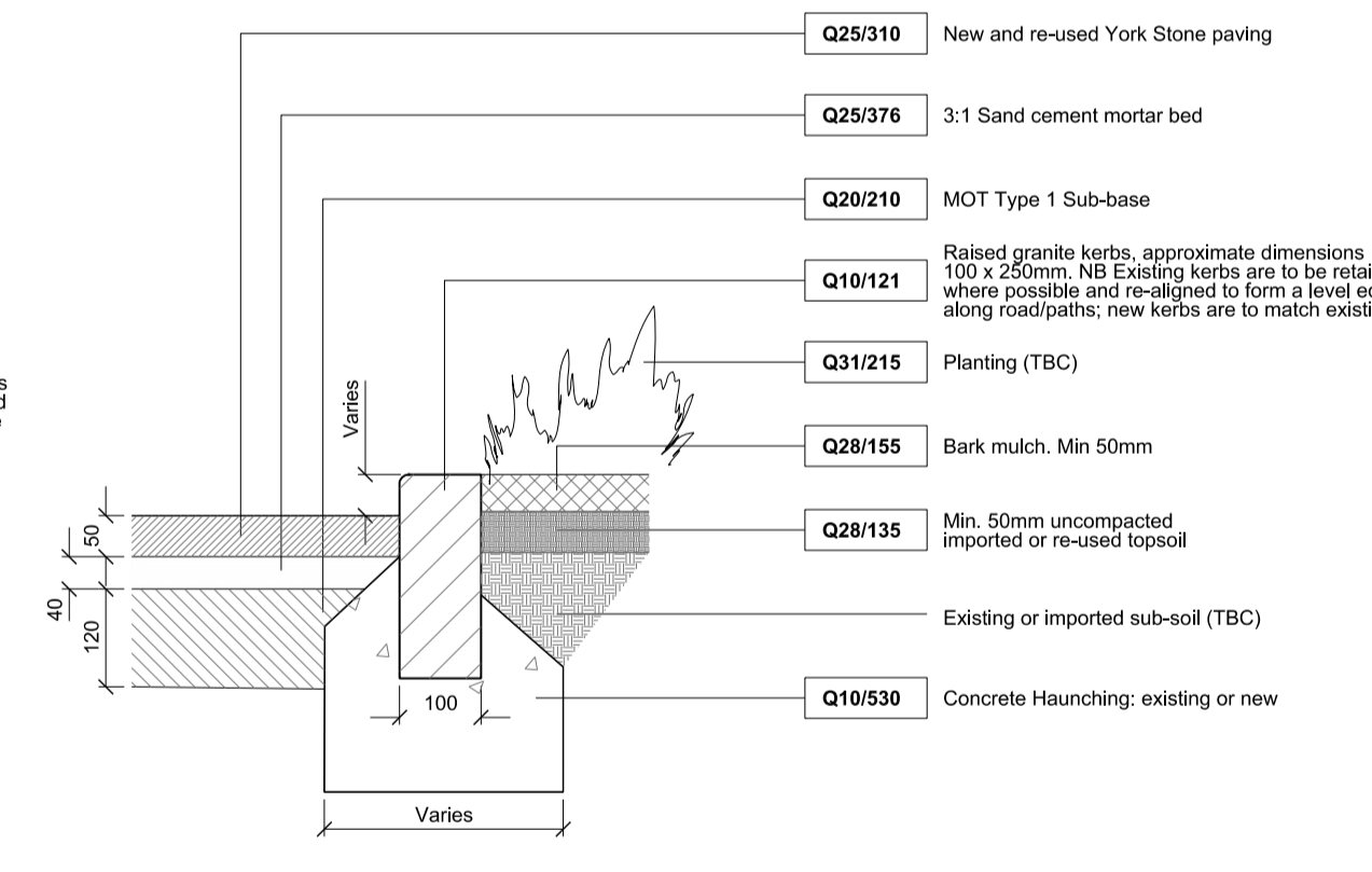
Granite Edge & York Stone Threshold Detail
