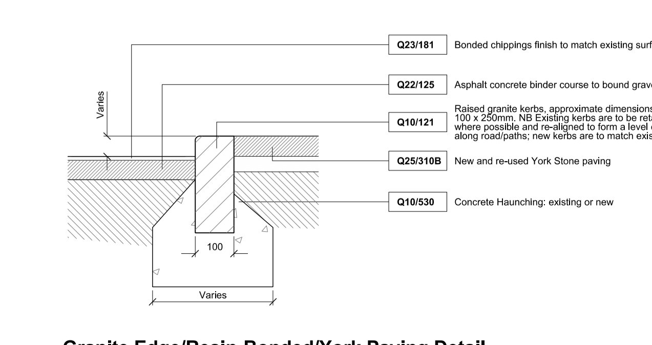
Granite Edge/Resin-Bonded/York Paving Detail
