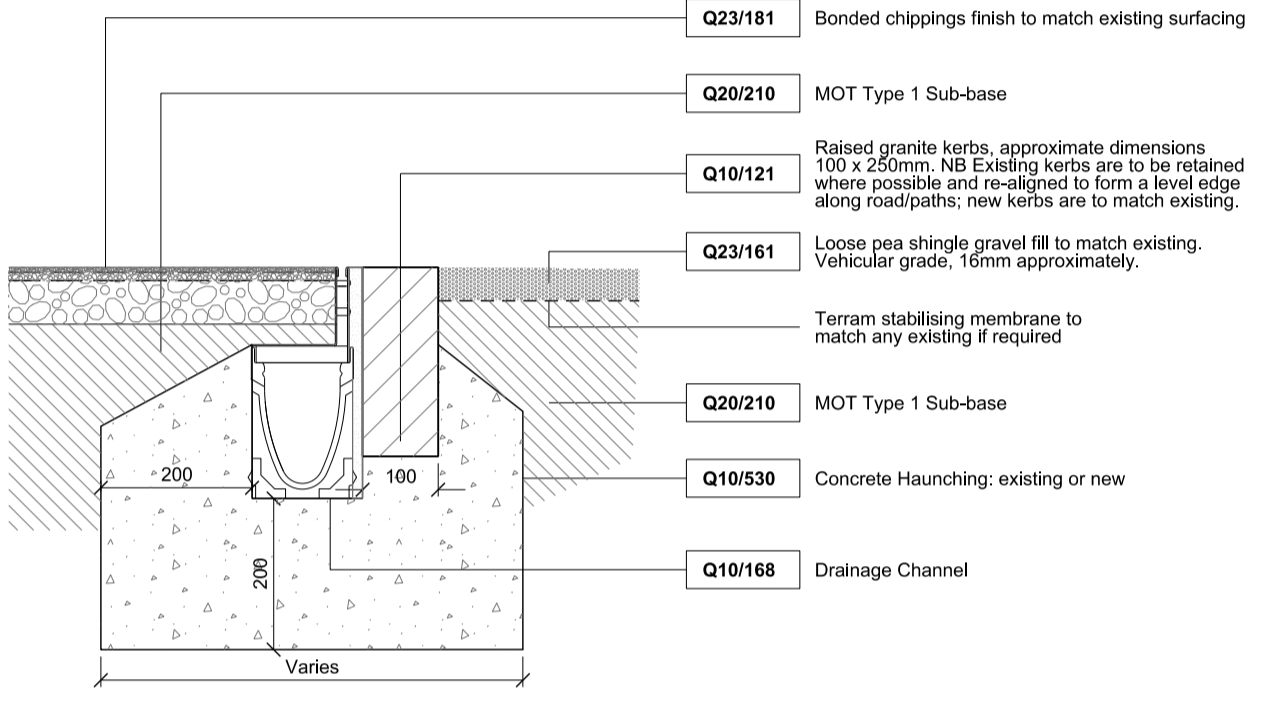
Granite Edge & Gravel/Bonded Gravel Detail
