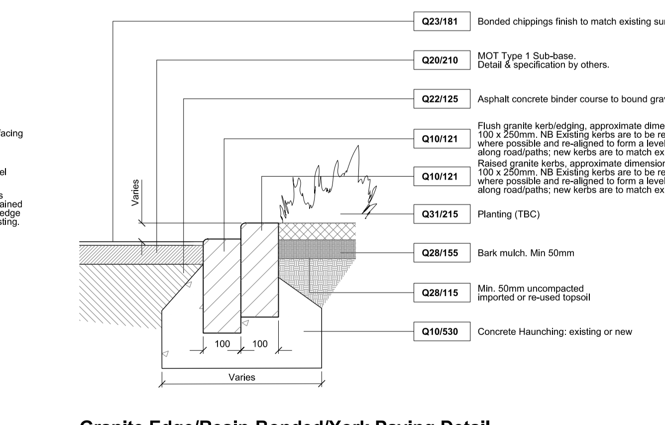
Granite Edge/Resin-Bonded/York Paving Detail
