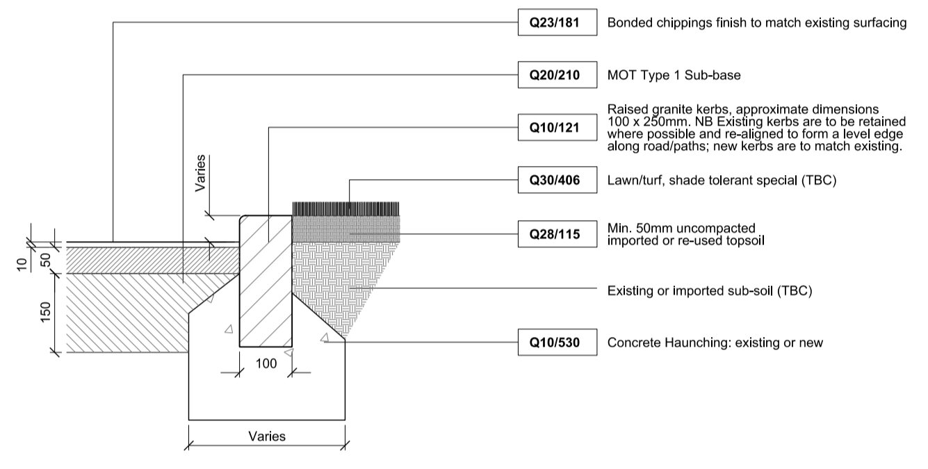
Granite Kerb/Edge Detail 2
