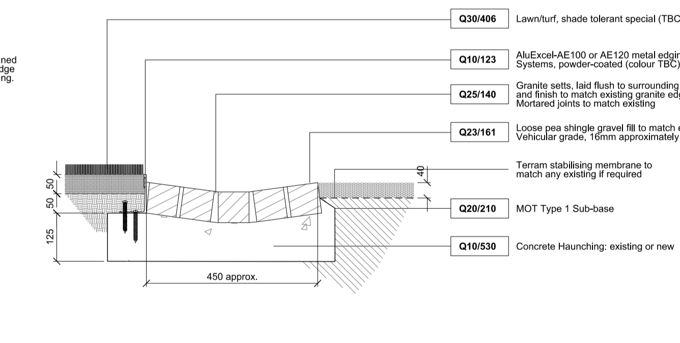
Granite open drainage channel detail
