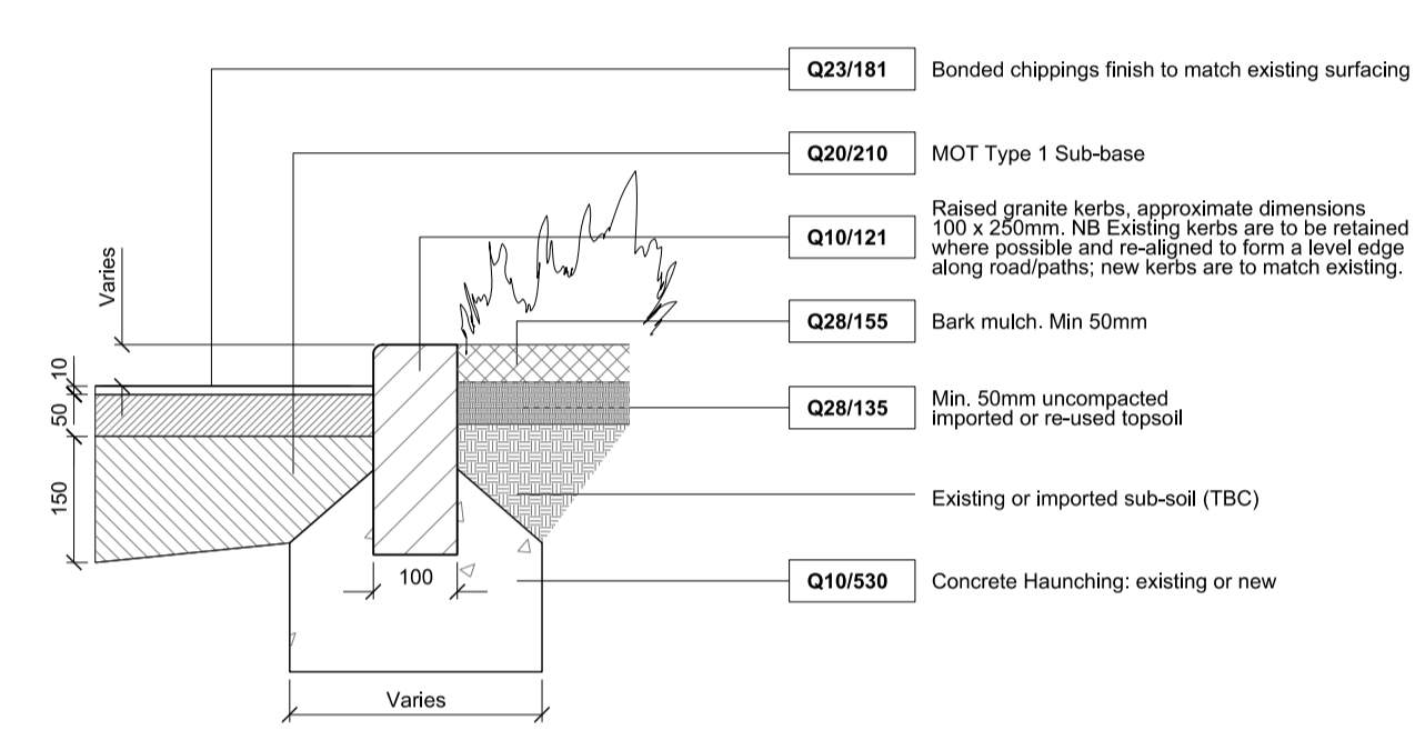
Granite Kerb/Edge Detail 3
