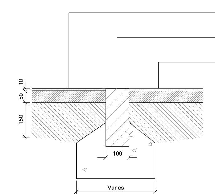
Junction Detail
