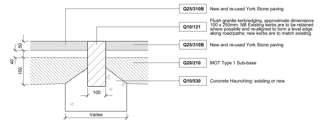
Granite Edge & York Stone Threshold Detail
