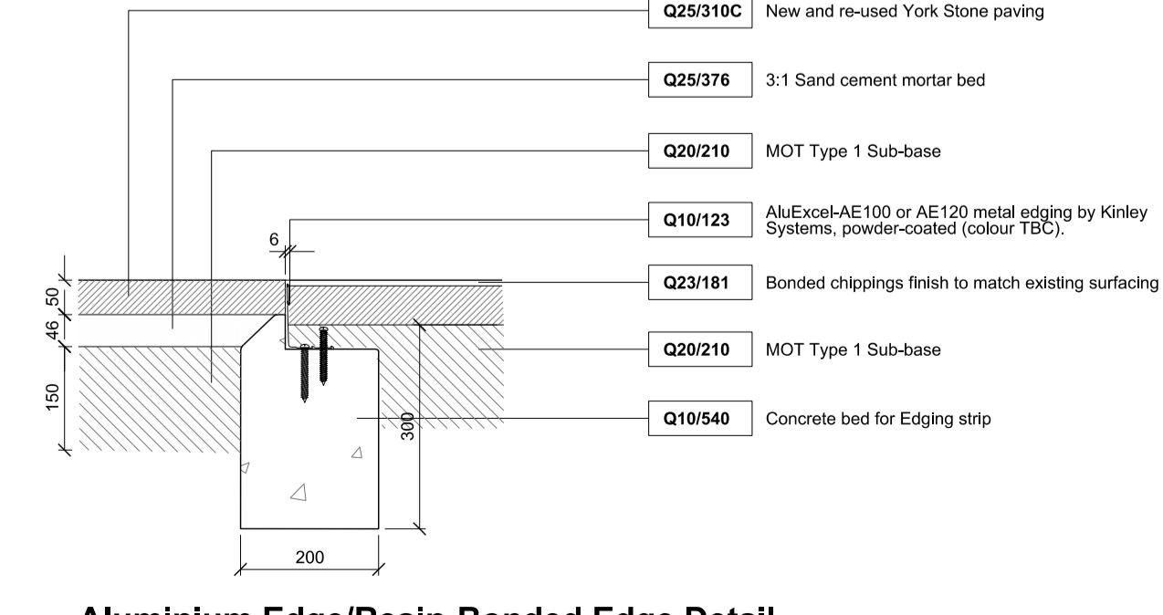
Aluminium Edge/Resin-Bonded Edge Detail
