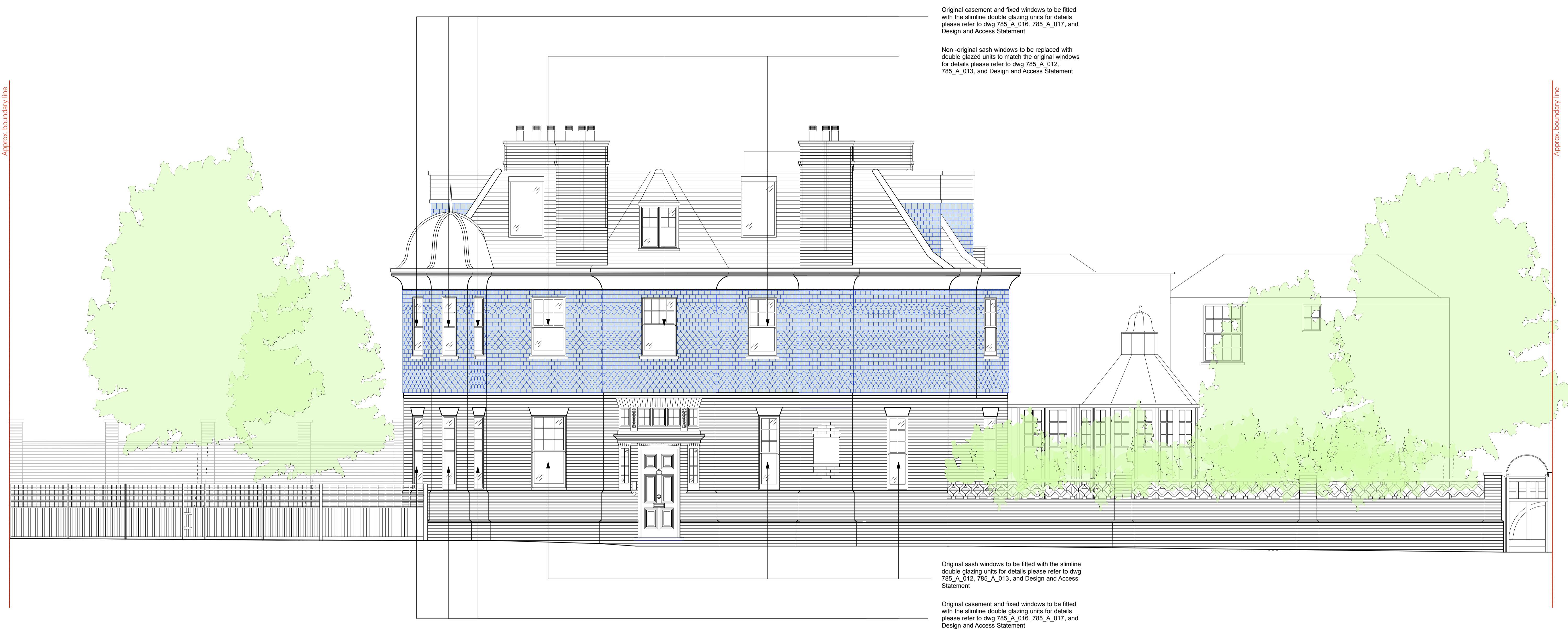
1 South West Elevation Scale: 1:50
