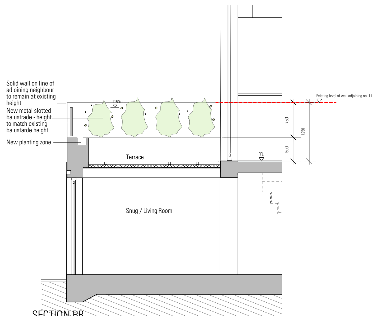
SECTION BB
