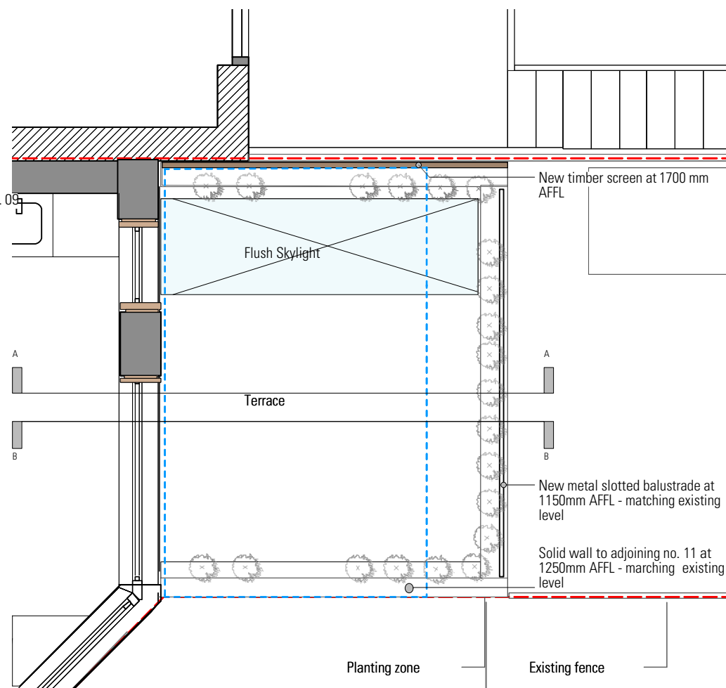
Plan of GF terrace
