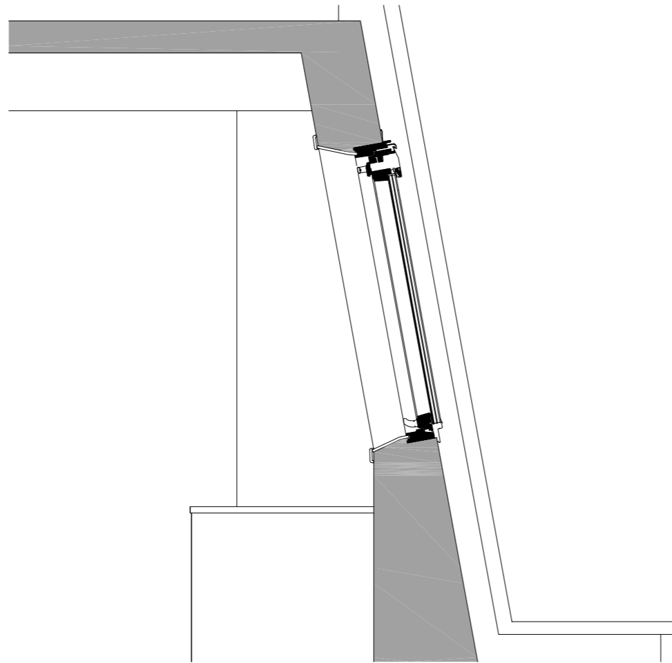
TYPICAL CONSERVATION ROOF WINDOW DETAIL 1:10@A3
