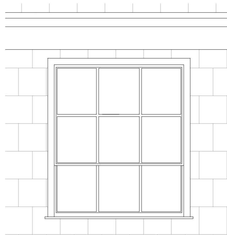
SLIDING SASH WINDOW ELEVATION 1:10@A3
