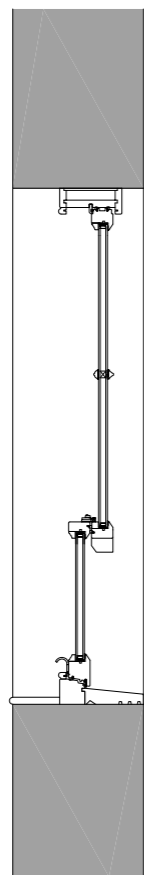
TYPICAL SLIDING SASH WINDOW DETAIL 1:10@A3
