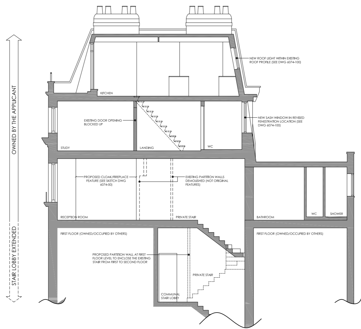
PROPOSED SECTION BB 1:50@A1
