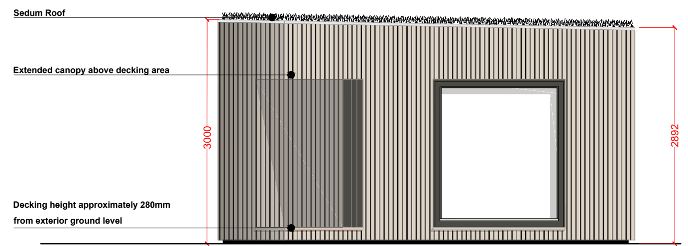
SOUTH WEST FACADE SCALE 1/50
