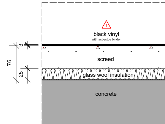
EXISTING FLOOR DETAIL SCALE 1:5 @ A3
