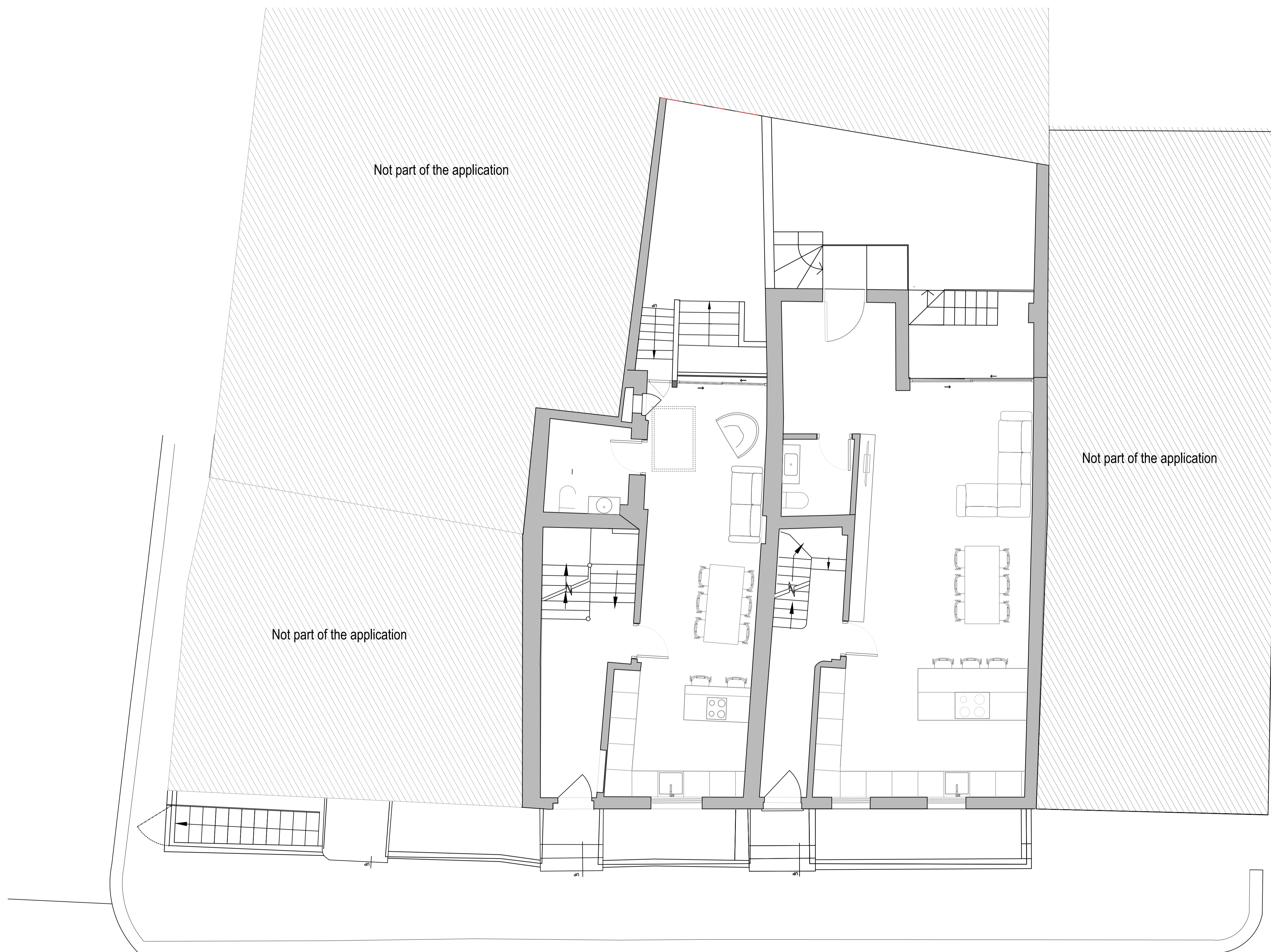
GROUND FLOOR PLAN E-0101
