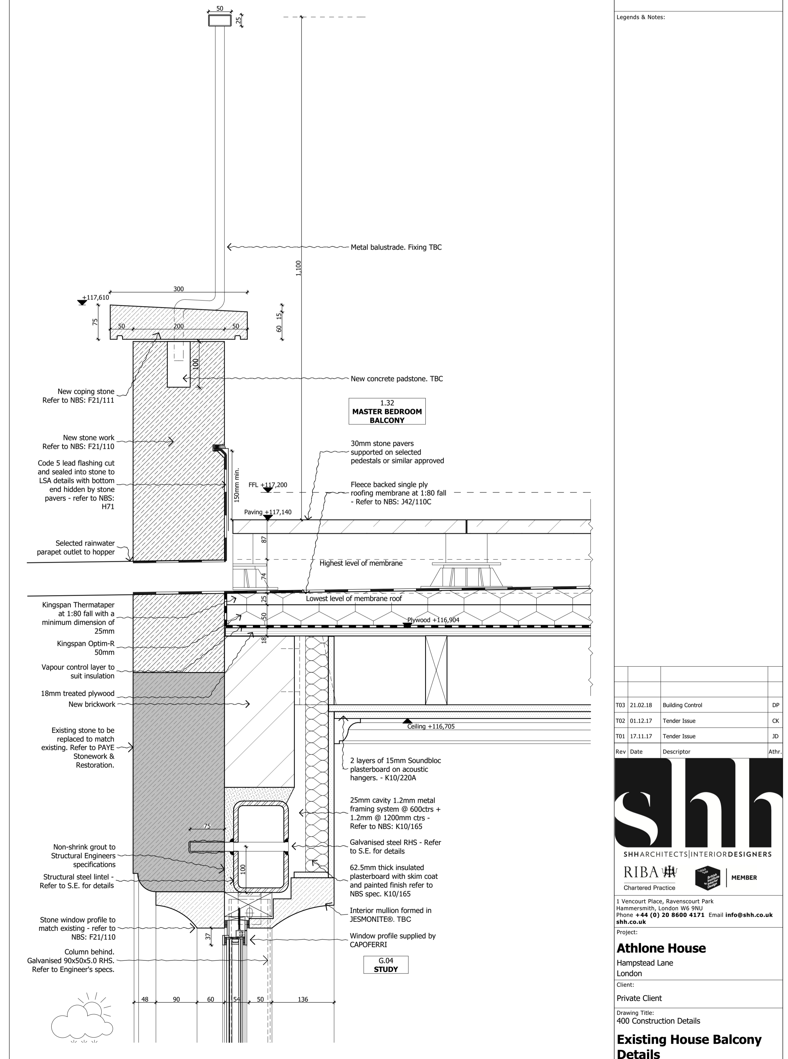
2 SCALE 1:5 @ A1; 1:10 @ A3 1.32 - MASTER BEDROOM BALCONY RAINWATER OUTLET DETAIL
