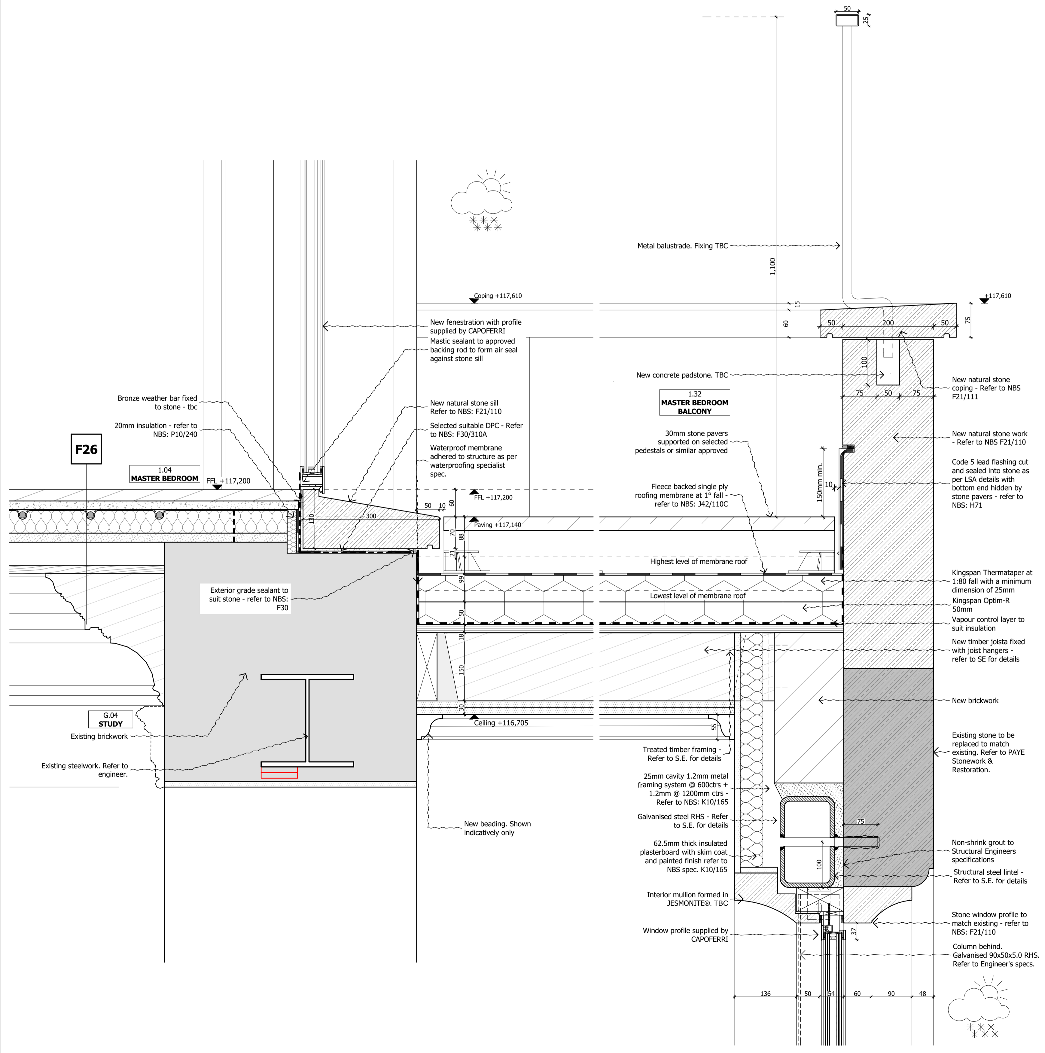
1 SCALE 1:5 @ A1; 1:10 @ A3 1.32 - MASTER BEDROOM BALCONY DETAIL (SECTION F-F)
