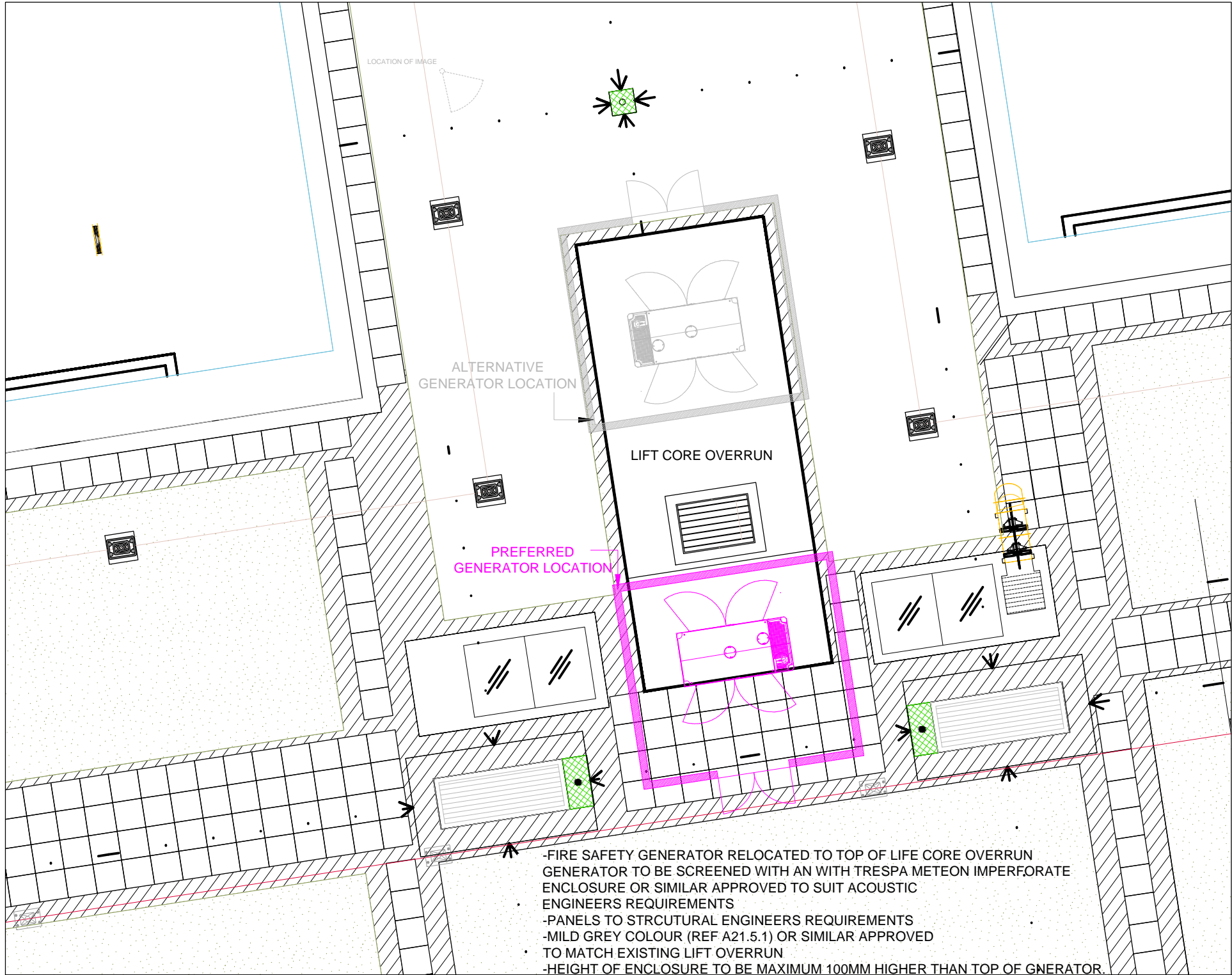
2 PROPOSED LOCATIONS PLAN
