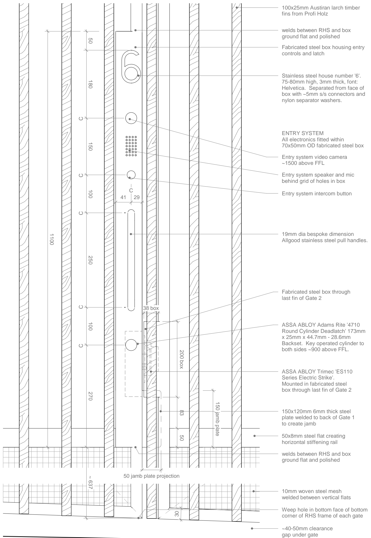
1 Entrance gate front elevation detail 1 : 5
